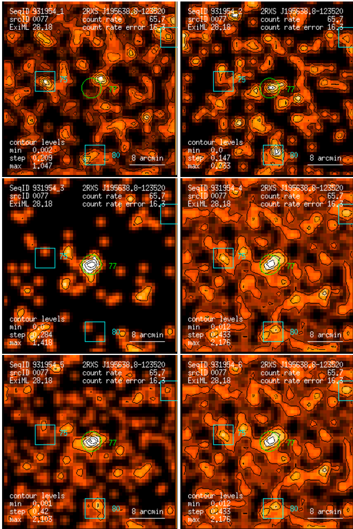
Figure 77: RASS 931954: detection 0077: band rate images, Gaussian filter: (1) PSPC channels 11 – 41, (2) 52 – 90, (3) 91 – 201, (4) 11 – 235, (5) 52 – 201, (6) 11 – 201. Broad band rates in counts/ks. Band rate contour levels in counts/ks/arcmin 2 .
