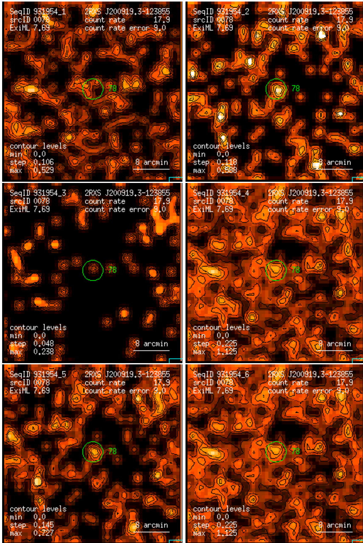
Figure 78: RASS 931954: detection 0078: band rate images, Gaussian filter: (1) PSPC channels 11 – 41, (2) 52 – 90, (3) 91 – 201, (4) 11 – 235, (5) 52 – 201, (6) 11 – 201. Broad band rates in counts/ks. Band rate contour levels in counts/ks/arcmin 2 .
