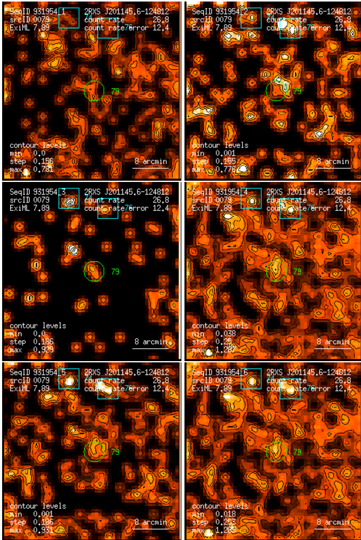
Figure 79: RASS 931954: detection 0079: band rate images, Gaussian filter: (1) PSPC channels 11 – 41, (2) 52 – 90, (3) 91 – 201, (4) 11 – 235, (5) 52 – 201, (6) 11 – 201. Broad band rates in counts/ks. Band rate contour levels in counts/ks/arcmin 2 .
