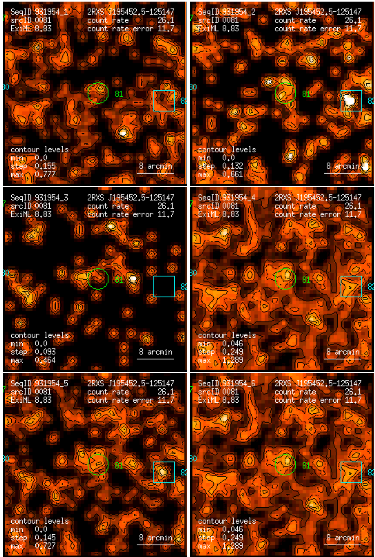
Figure 81: RASS 931954: detection 0081: band rate images, Gaussian filter: (1) PSPC channels 11 – 41, (2) 52 – 90, (3) 91 – 201, (4) 11 – 235, (5) 52 – 201, (6) 11 – 201. Broad band rates in counts/ks. Band rate contour levels in counts/ks/arcmin 2 .
