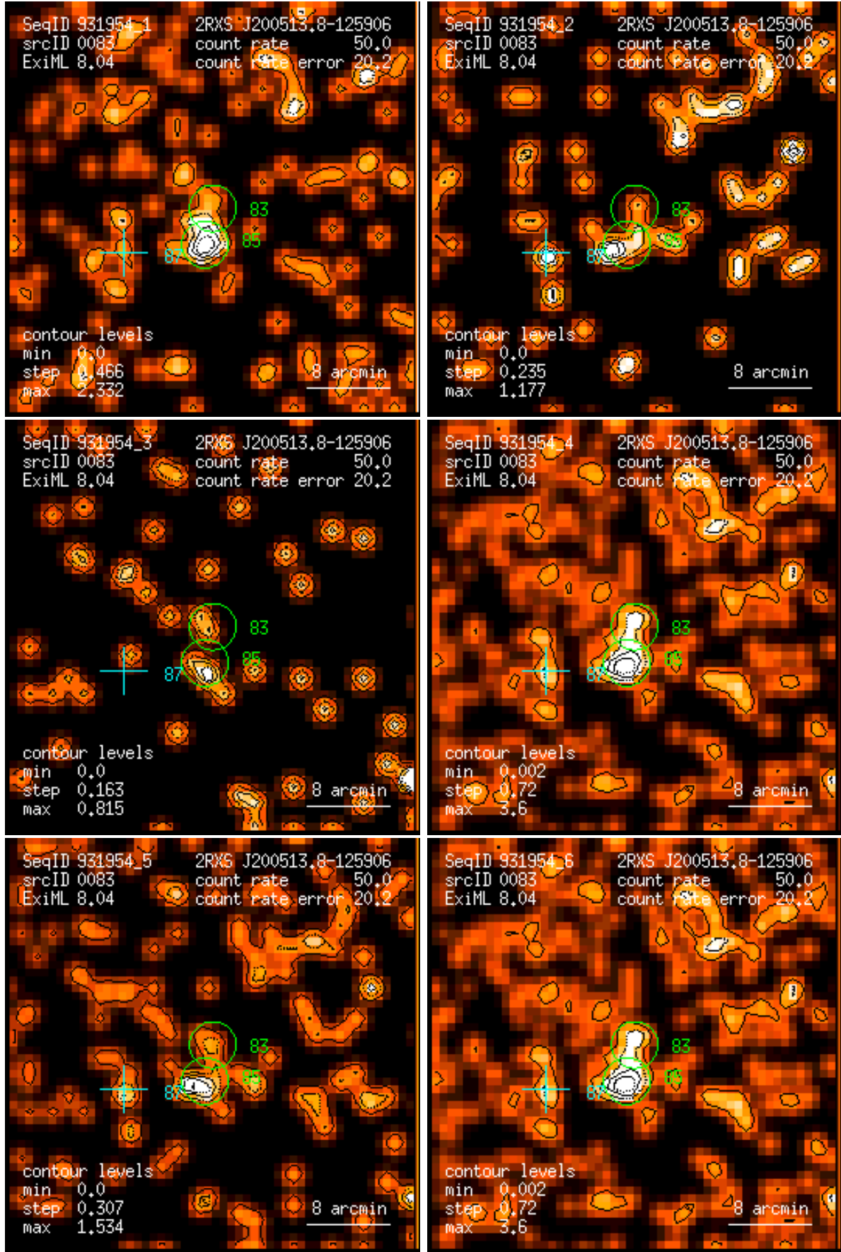
Figure 83: RASS 931954: detection 0083: band rate images, Gaussian filter: (1) PSPC channels 11 – 41, (2) 52 – 90, (3) 91 – 201, (4) 11 – 235, (5) 52 – 201, (6) 11 – 201. Broad band rates in counts/ks. Band rate contour levels in counts/ks/arcmin 2 .
