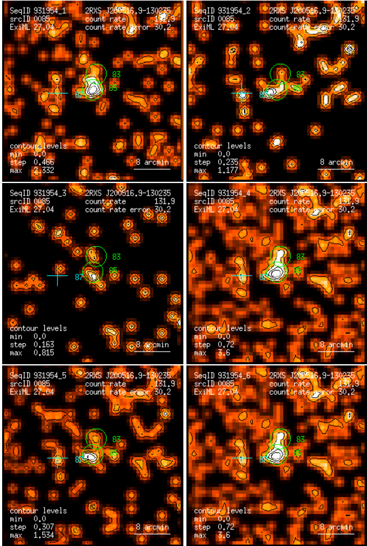
Figure 85: RASS 931954: detection 0085: band rate images, Gaussian filter: (1) PSPC channels 11 – 41, (2) 52 – 90, (3) 91 – 201, (4) 11 – 235, (5) 52 – 201, (6) 11 – 201. Broad band rates in counts/ks. Band rate contour levels in counts/ks/arcmin 2 .
