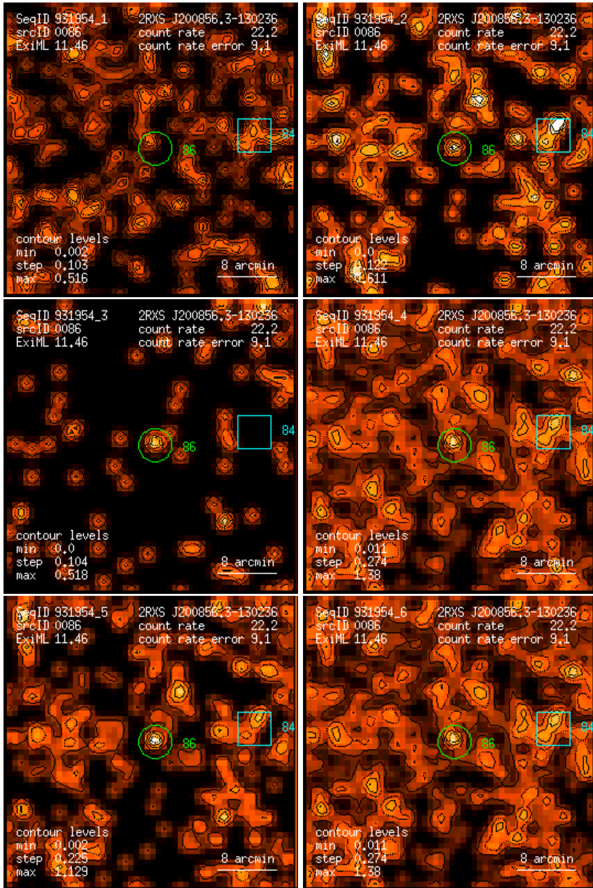
Figure 86: RASS 931954: detection 0086: band rate images, Gaussian filter: (1) PSPC channels 11 – 41, (2) 52 – 90, (3) 91 – 201, (4) 11 – 235, (5) 52 – 201, (6) 11 – 201. Broad band rates in counts/ks. Band rate contour levels in counts/ks/arcmin 2 .
