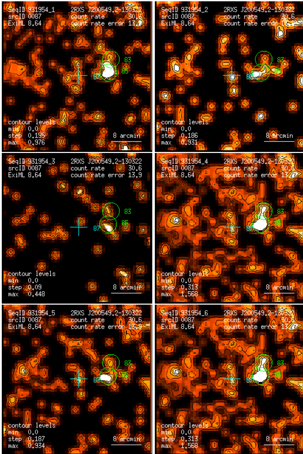
Figure 87: RASS 931954: detection 0087: band rate images, Gaussian filter: (1) PSPC channels 11 – 41, (2) 52 – 90, (3) 91 – 201, (4) 11 – 235, (5) 52 – 201, (6) 11 – 201. Broad band rates in counts/ks. Band rate contour levels in counts/ks/arcmin 2 .
