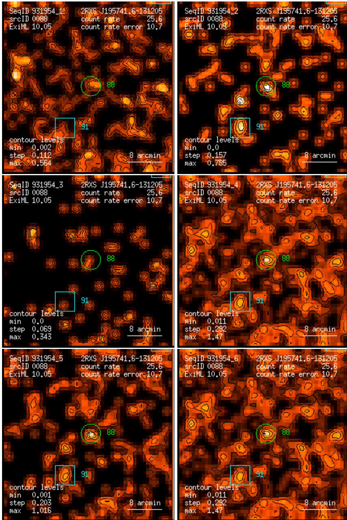
Figure 88: RASS 931954: detection 0088: band rate images, Gaussian filter: (1) PSPC channels 11 – 41, (2) 52 – 90, (3) 91 – 201, (4) 11 – 235, (5) 52 – 201, (6) 11 – 201. Broad band rates in counts/ks. Band rate contour levels in counts/ks/arcmin 2 .
