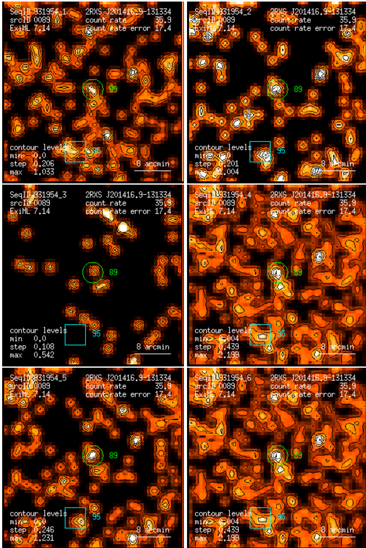
Figure 89: RASS 931954: detection 0089: band rate images, Gaussian filter: (1) PSPC channels 11 – 41, (2) 52 – 90, (3) 91 – 201, (4) 11 – 235, (5) 52 – 201, (6) 11 – 201. Broad band rates in counts/ks. Band rate contour levels in counts/ks/arcmin 2 .
