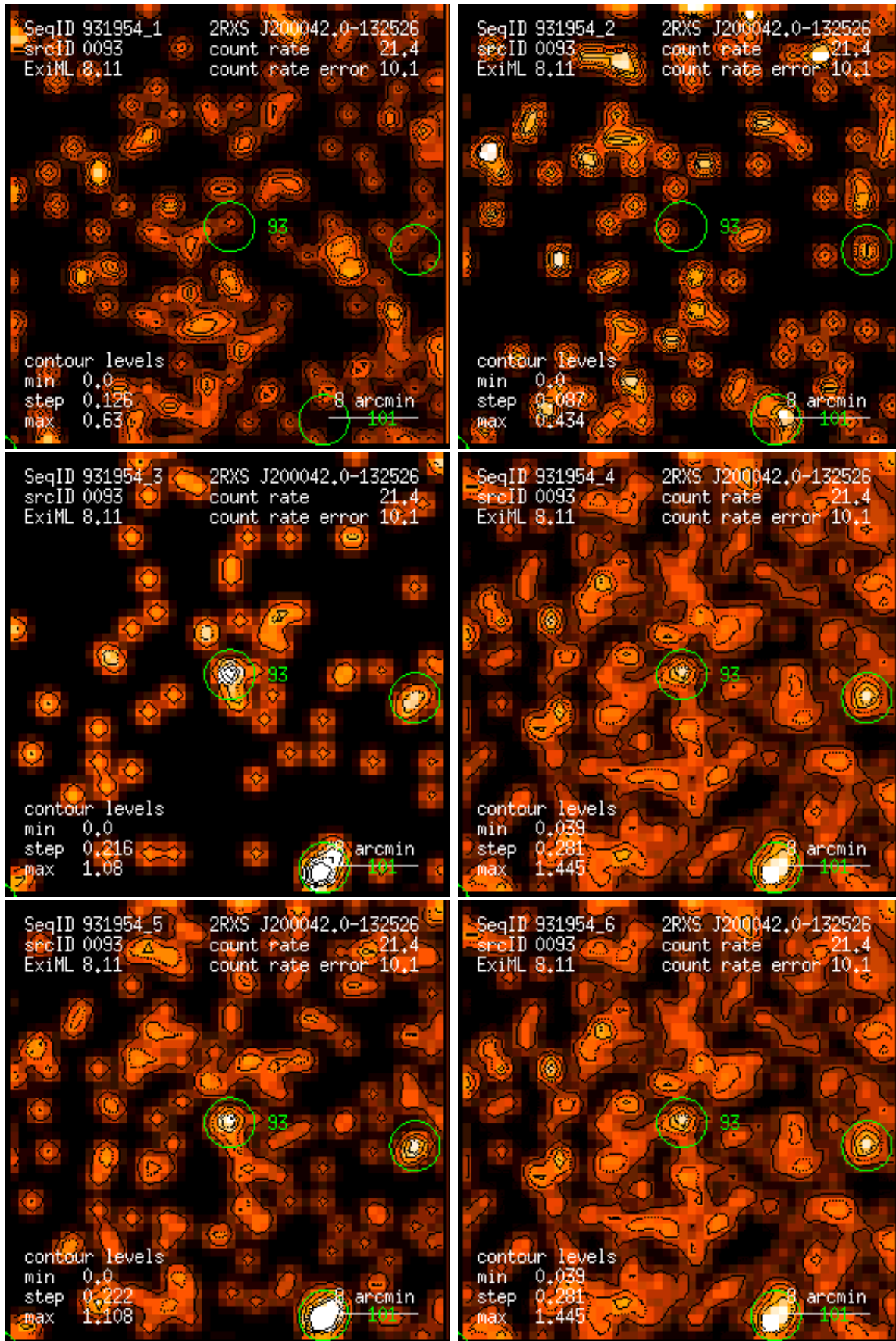
Figure 93: RASS 931954: detection 0093: band rate images, Gaussian filter: (1) PSPC channels 11 – 41, (2) 52 – 90, (3) 91 – 201, (4) 11 – 235, (5) 52 – 201, (6) 11 – 201. Broad band rates in counts/ks. Band rate contour levels in counts/ks/arcmin 2 .
