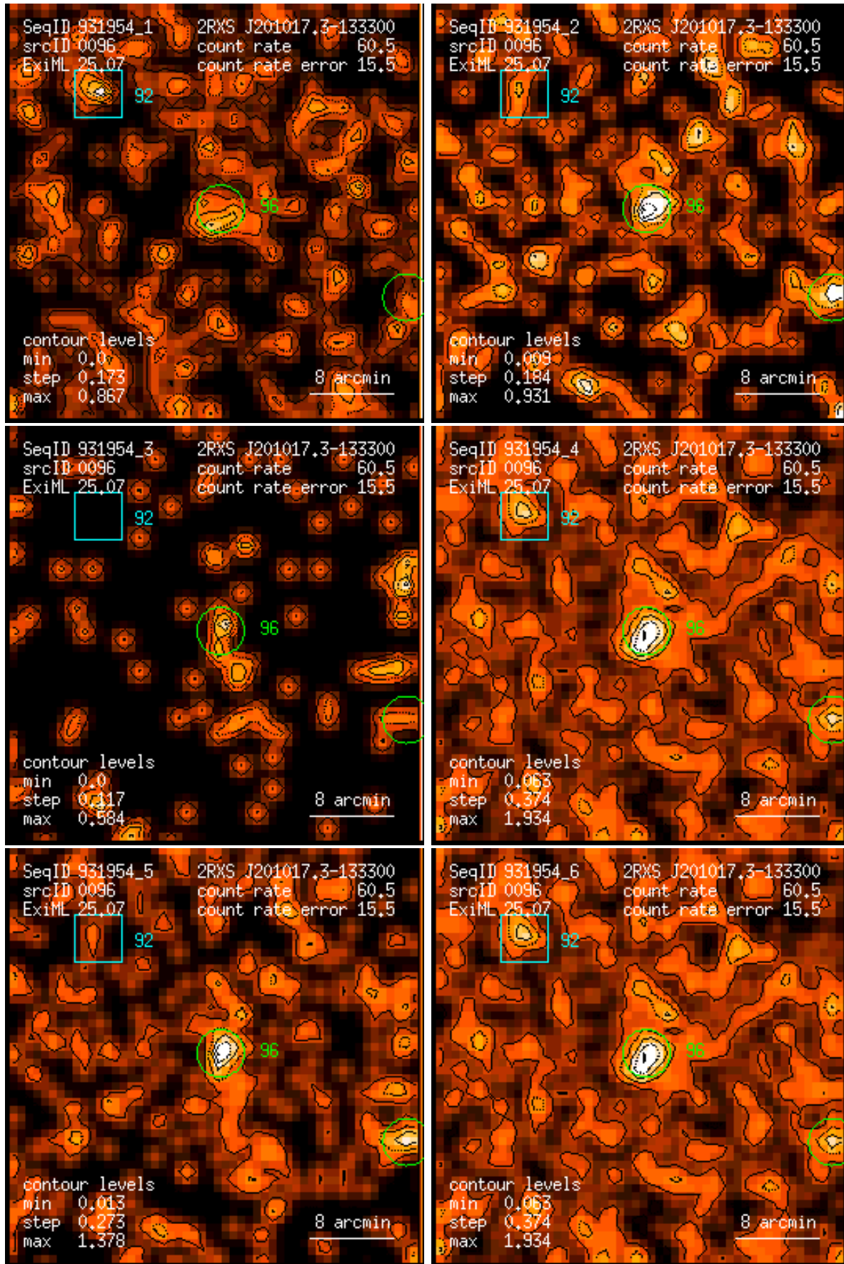
Figure 96: RASS 931954: detection 0096: band rate images, Gaussian filter: (1) PSPC channels 11 – 41, (2) 52 – 90, (3) 91 – 201, (4) 11 – 235, (5) 52 – 201, (6) 11 – 201. Broad band rates in counts/ks. Band rate contour levels in counts/ks/arcmin 2 .
