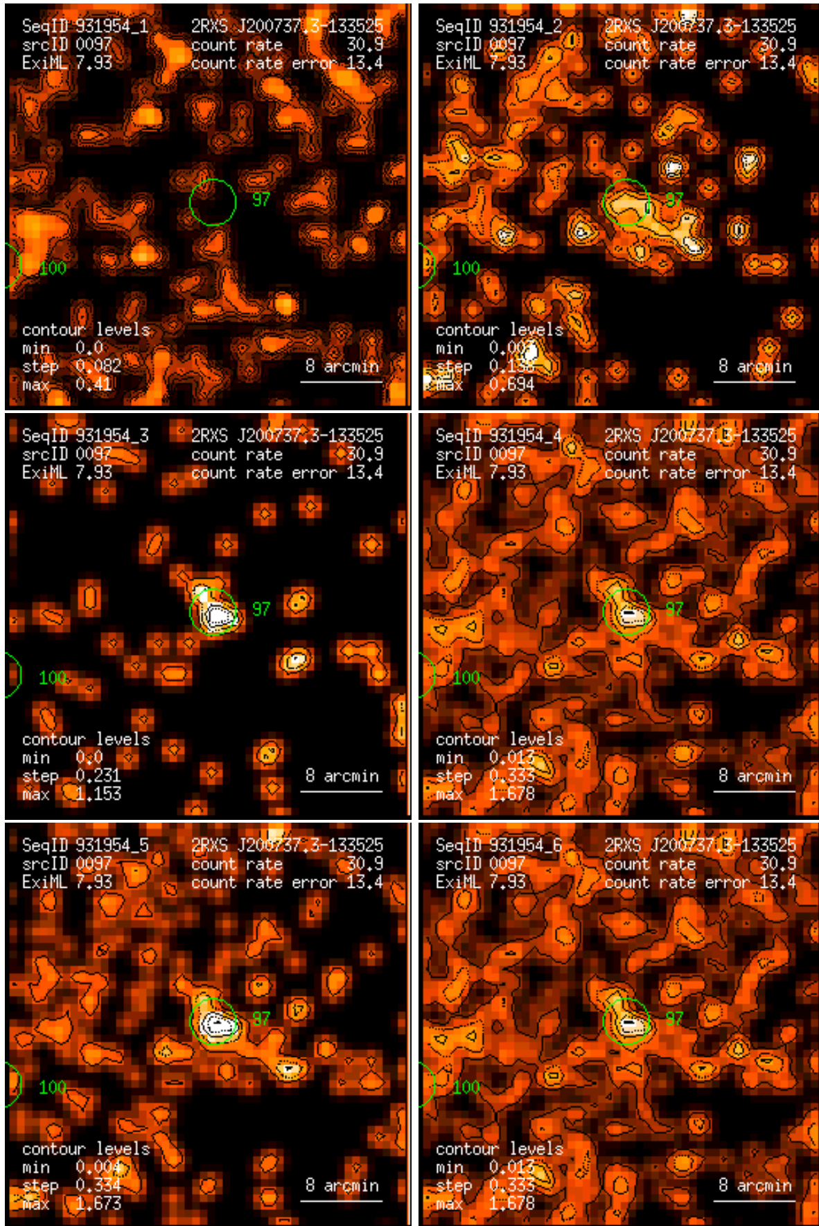
Figure 97: RASS 931954: detection 0097: band rate images, Gaussian filter: (1) PSPC channels 11 – 41, (2) 52 – 90, (3) 91 – 201, (4) 11 – 235, (5) 52 – 201, (6) 11 – 201. Broad band rates in counts/ks. Band rate contour levels in counts/ks/arcmin 2 .
