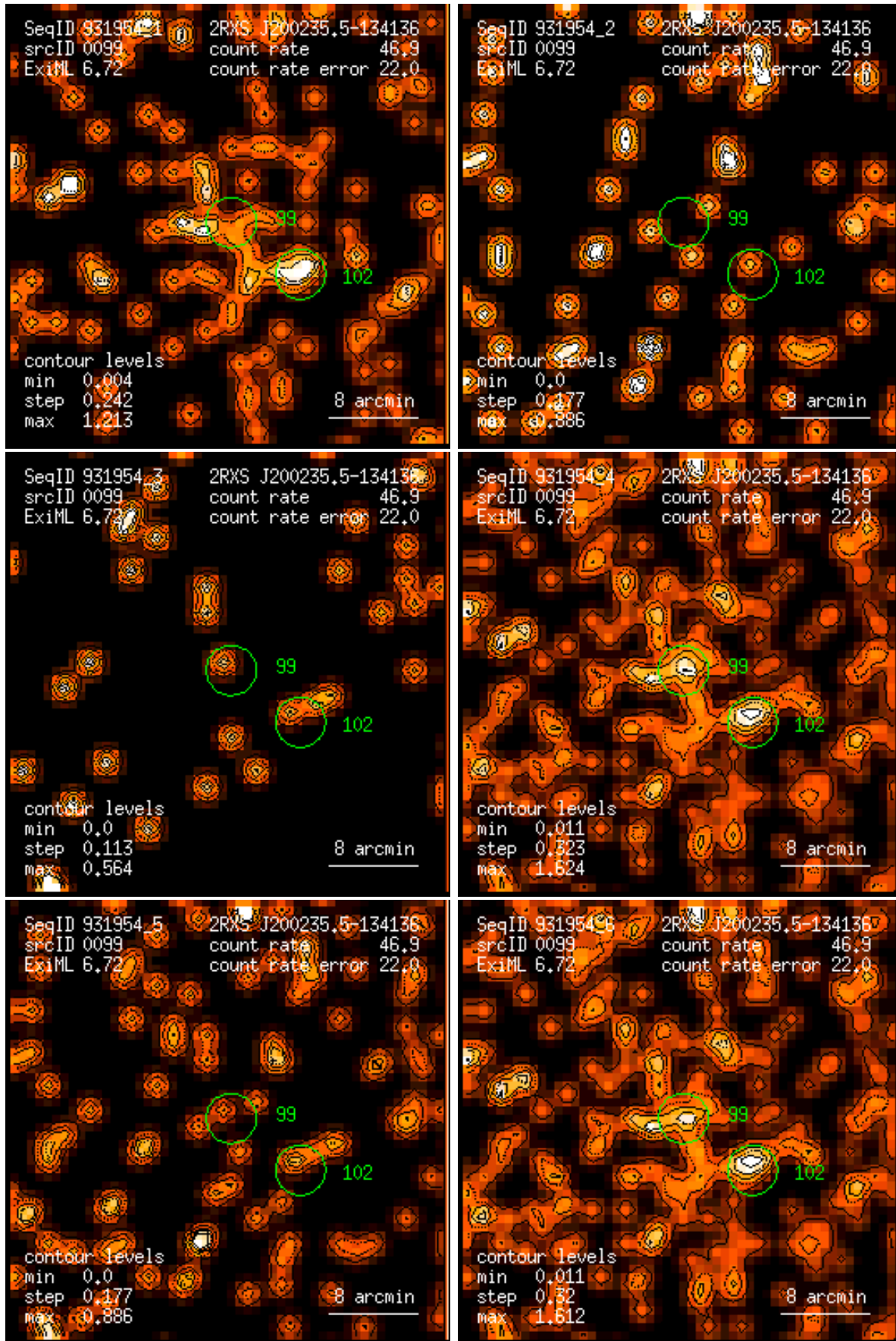
Figure 99: RASS 931954: detection 0099: band rate images, Gaussian filter: (1) PSPC channels 11 – 41, (2) 52 – 90, (3) 91 – 201, (4) 11 – 235, (5) 52 – 201, (6) 11 – 201. Broad band rates in counts/ks. Band rate contour levels in counts/ks/arcmin 2 .
