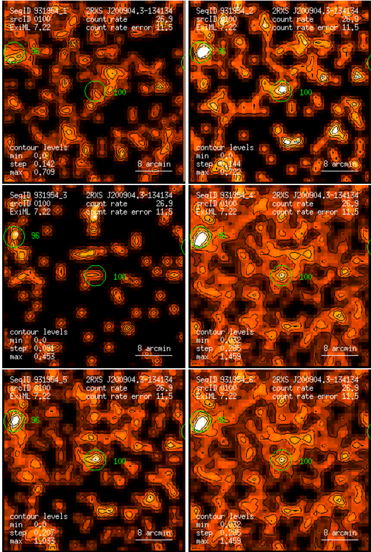
Figure 100: RASS 931954: detection 0100: band rate images, Gaussian filter: (1) PSPC channels 11 – 41, (2) 52 – 90, (3) 91 – 201, (4) 11 – 235, (5) 52 – 201, (6) 11 – 201. Broad band rates in counts/ks. Band rate contour levels in counts/ks/arcmin 2 .
