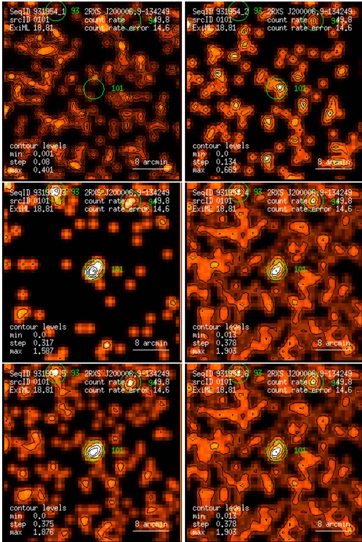
Figure 101: RASS 931954: detection 0101: band rate images, Gaussian filter: (1) PSPC channels 11 – 41, (2) 52 – 90, (3) 91 – 201, (4) 11 – 235, (5) 52 – 201, (6) 11 – 201. Broad band rates in counts/ks. Band rate contour levels in counts/ks/arcmin 2 .
