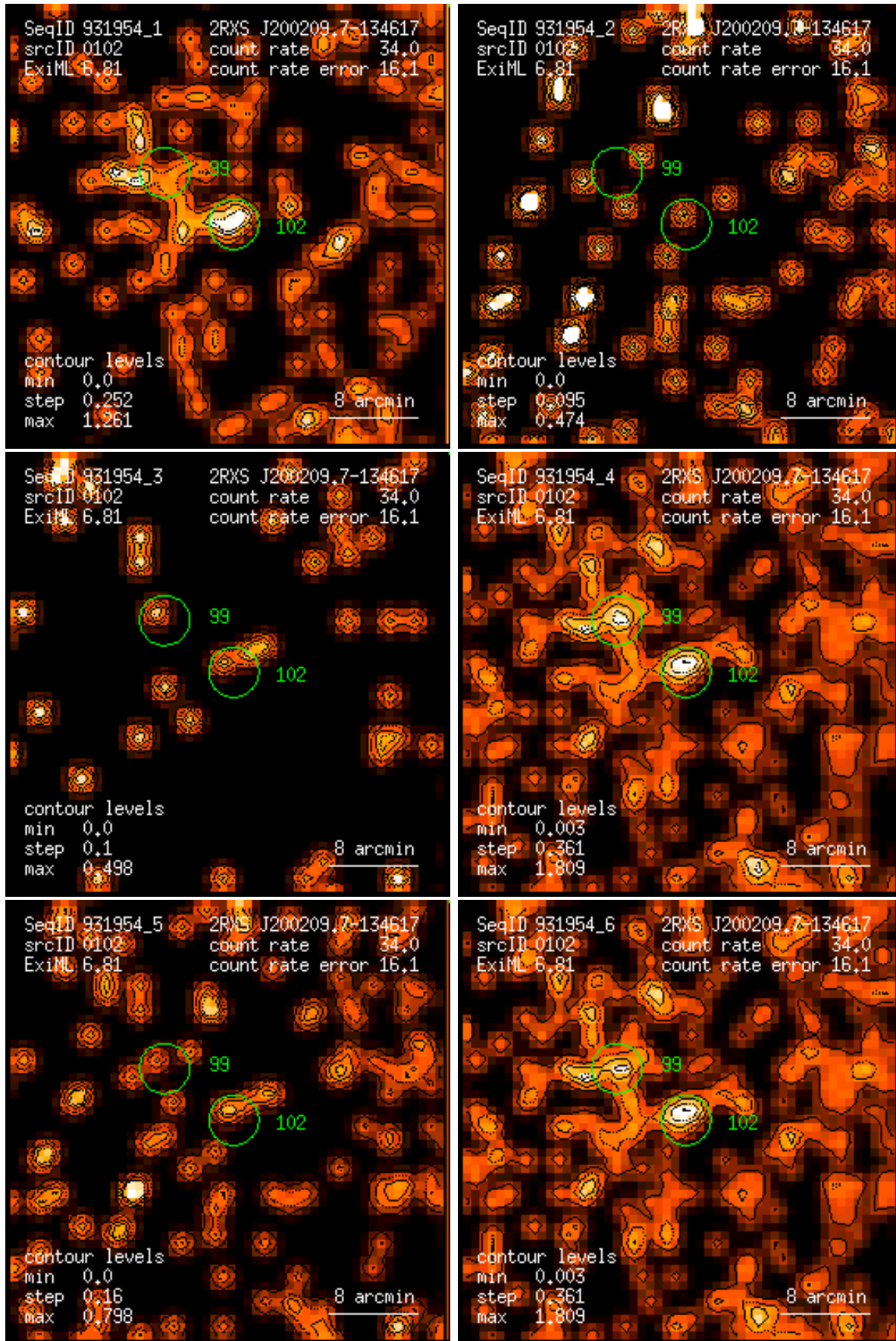
Figure 102: RASS 931954: detection 0102: band rate images, Gaussian filter: (1) PSPC channels 11 – 41, (2) 52 – 90, (3) 91 – 201, (4) 11 – 235, (5) 52 – 201, (6) 11 – 201. Broad band rates in counts/ks. Band rate contour levels in counts/ks/arcmin 2 .
