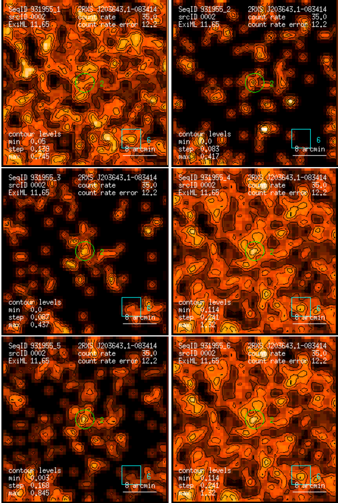
Figure 2: RASS 931955: detection 0002: band rate images, Gaussian filter: (1) PSPC channels 11 – 41, (2) 52 – 90, (3) 91 – 201, (4) 11 – 235, (5) 52 – 201, (6) 11 – 201. Broad band rates in counts/ks. Band rate contour levels in counts/ks/arcmin 2 .
