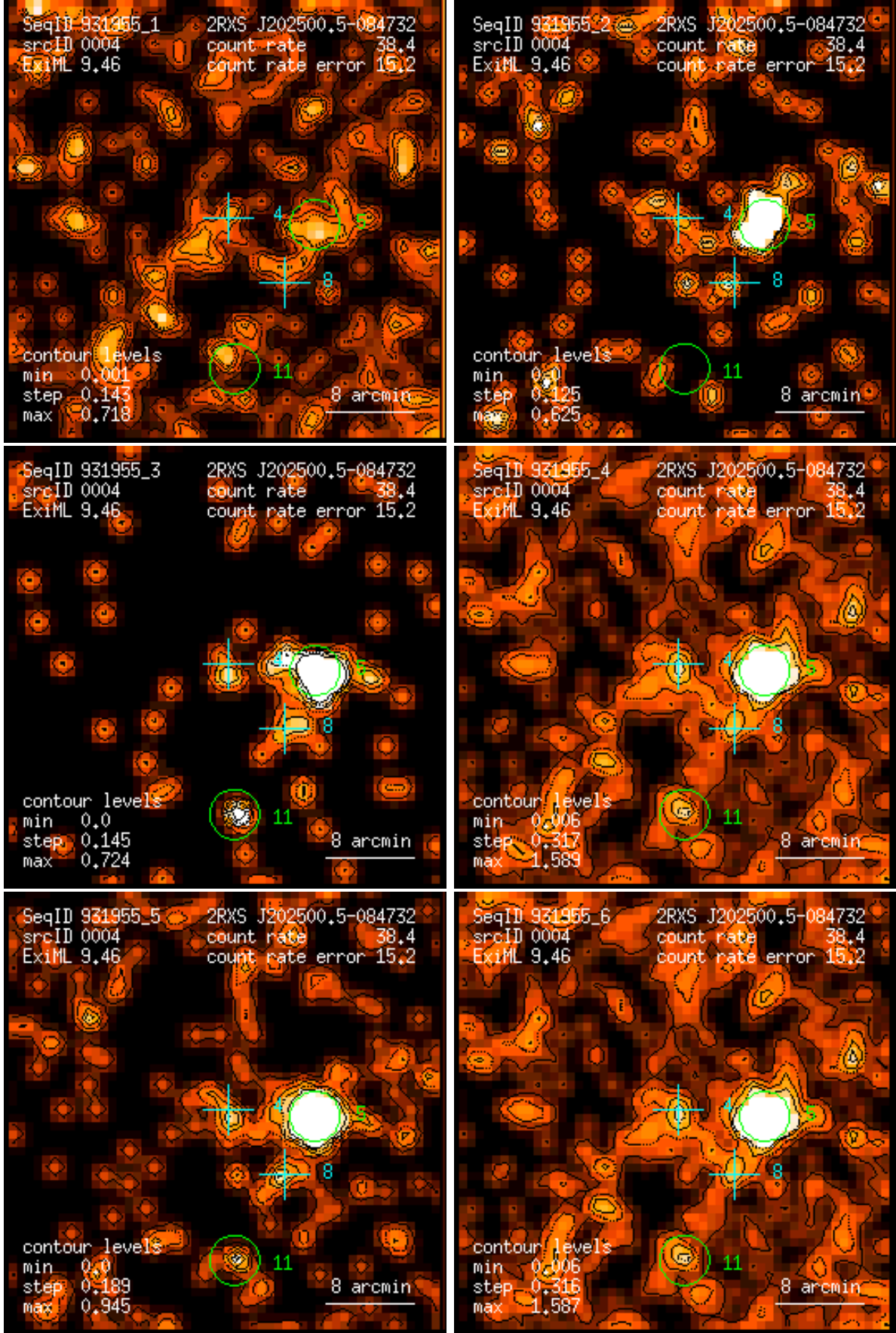
Figure 4: RASS 931955: detection 0004: band rate images, Gaussian filter: (1) PSPC channels 11 – 41, (2) 52 – 90, (3) 91 – 201, (4) 11 – 235, (5) 52 – 201, (6) 11 – 201. Broad band rates in counts/ks. Band rate contour levels in counts/ks/arcmin 2 .
