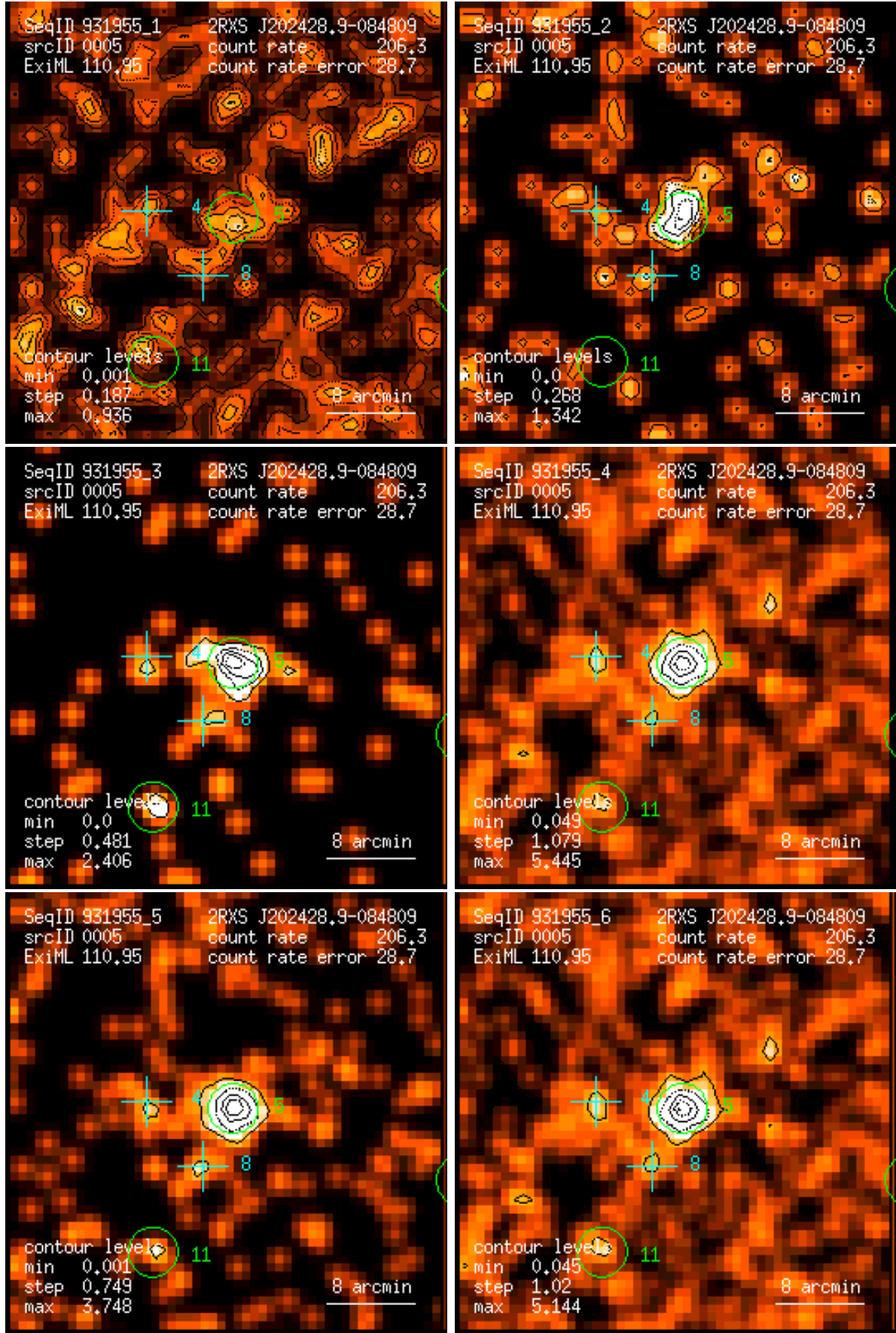
Figure 5: RASS 931955: detection 0005: band rate images, Gaussian filter: (1) PSPC channels 11 – 41, (2) 52 – 90, (3) 91 – 201, (4) 11 – 235, (5) 52 – 201, (6) 11 – 201. Broad band rates in counts/ks. Band rate contour levels in counts/ks/arcmin 2 .
