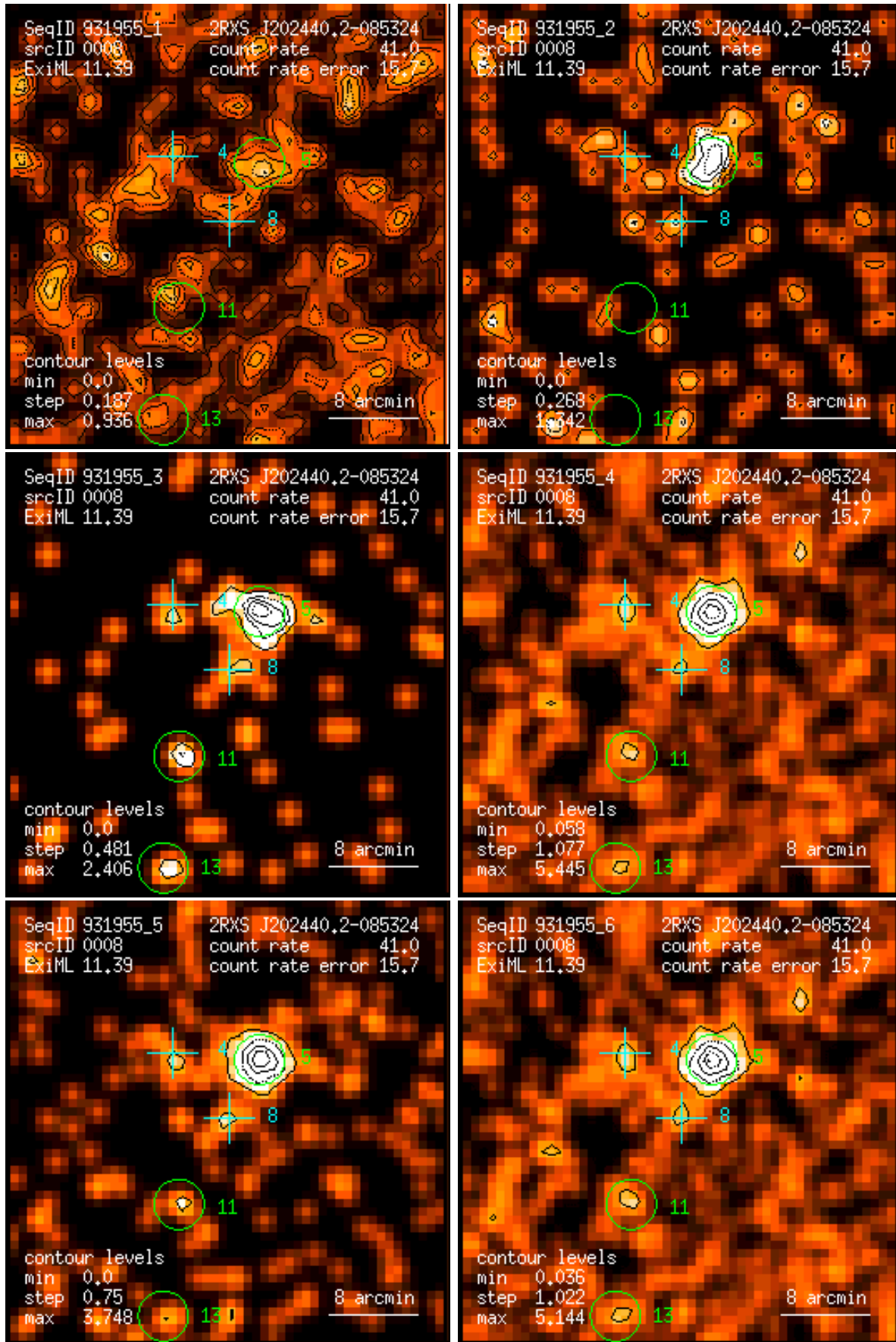
Figure 8: RASS 931955: detection 0008: band rate images, Gaussian filter: (1) PSPC channels 11 – 41, (2) 52 – 90, (3) 91 – 201, (4) 11 – 235, (5) 52 – 201, (6) 11 – 201. Broad band rates in counts/ks. Band rate contour levels in counts/ks/arcmin 2 .
