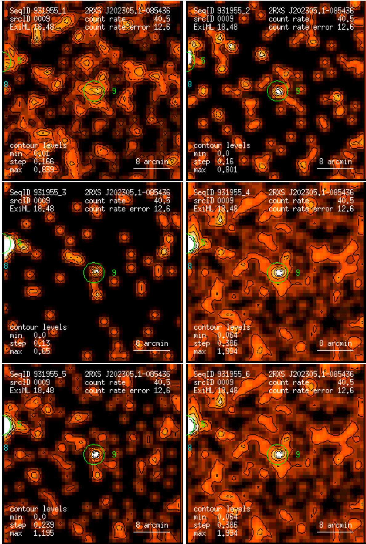
Figure 9: RASS 931955: detection 0009: band rate images, Gaussian filter: (1) PSPC channels 11 – 41, (2) 52 – 90, (3) 91 – 201, (4) 11 – 235, (5) 52 – 201, (6) 11 – 201. Broad band rates in counts/ks. Band rate contour levels in counts/ks/arcmin 2 .
