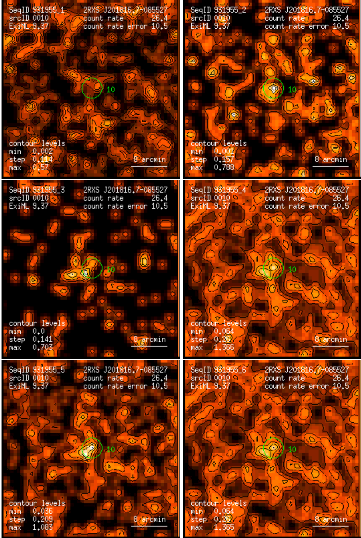
Figure 10: RASS 931955: detection 0010: band rate images, Gaussian filter: (1) PSPC channels 11 – 41, (2) 52 – 90, (3) 91 – 201, (4) 11 – 235, (5) 52 – 201, (6) 11 – 201. Broad band rates in counts/ks. Band rate contour levels in counts/ks/arcmin 2 .
