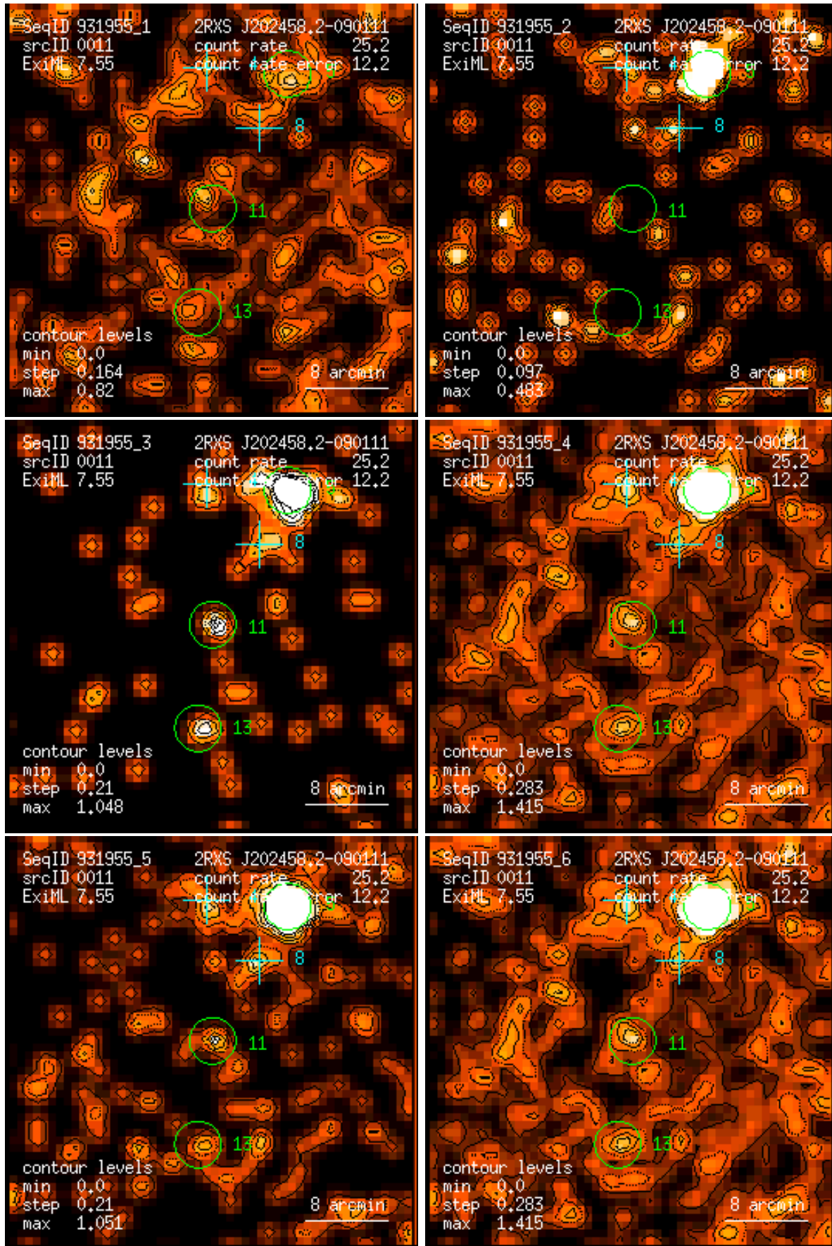
Figure 11: RASS 931955: detection 0011: band rate images, Gaussian filter: (1) PSPC channels 11 – 41, (2) 52 – 90, (3) 91 – 201, (4) 11 – 235, (5) 52 – 201, (6) 11 – 201. Broad band rates in counts/ks. Band rate contour levels in counts/ks/arcmin 2 .
