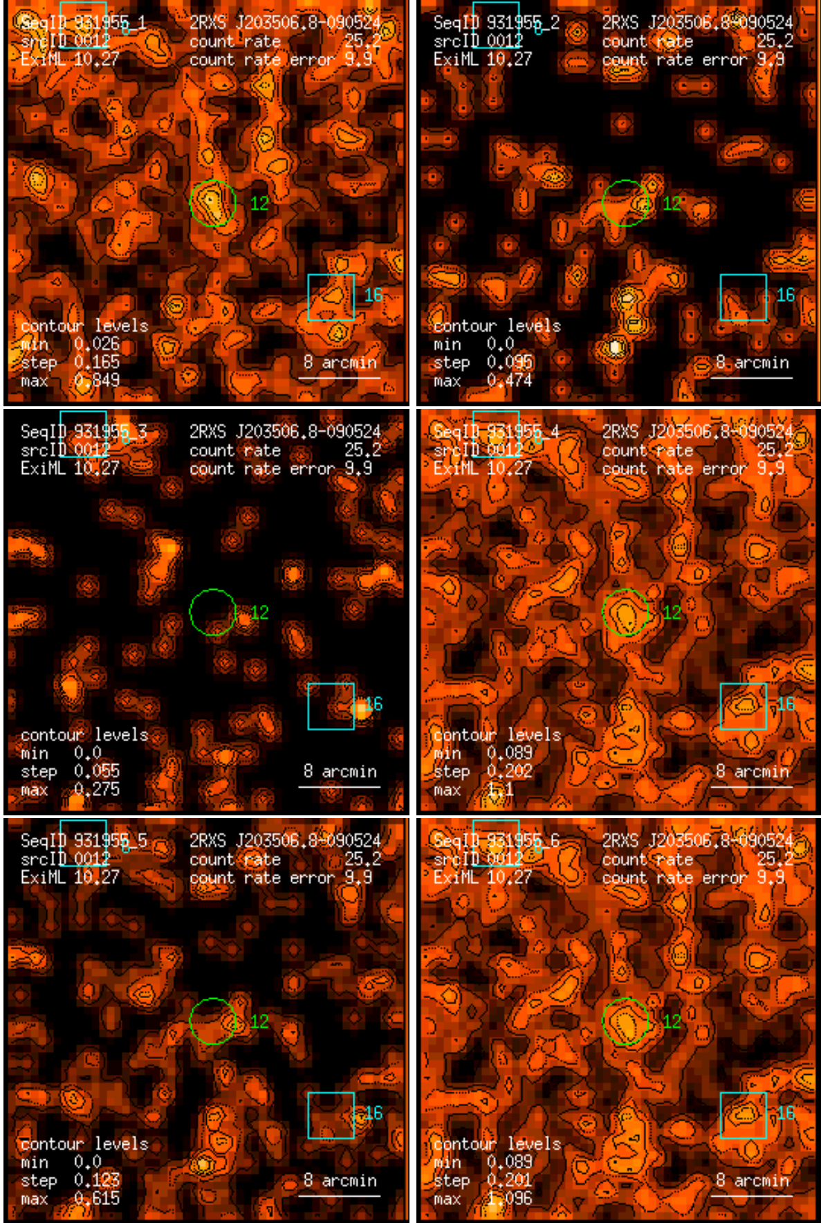
Figure 12: RASS 931955: detection 0012: band rate images, Gaussian filter: (1) PSPC channels 11 – 41, (2) 52 – 90, (3) 91 – 201, (4) 11 – 235, (5) 52 – 201, (6) 11 – 201. Broad band rates in counts/ks. Band rate contour levels in counts/ks/arcmin 2 .
