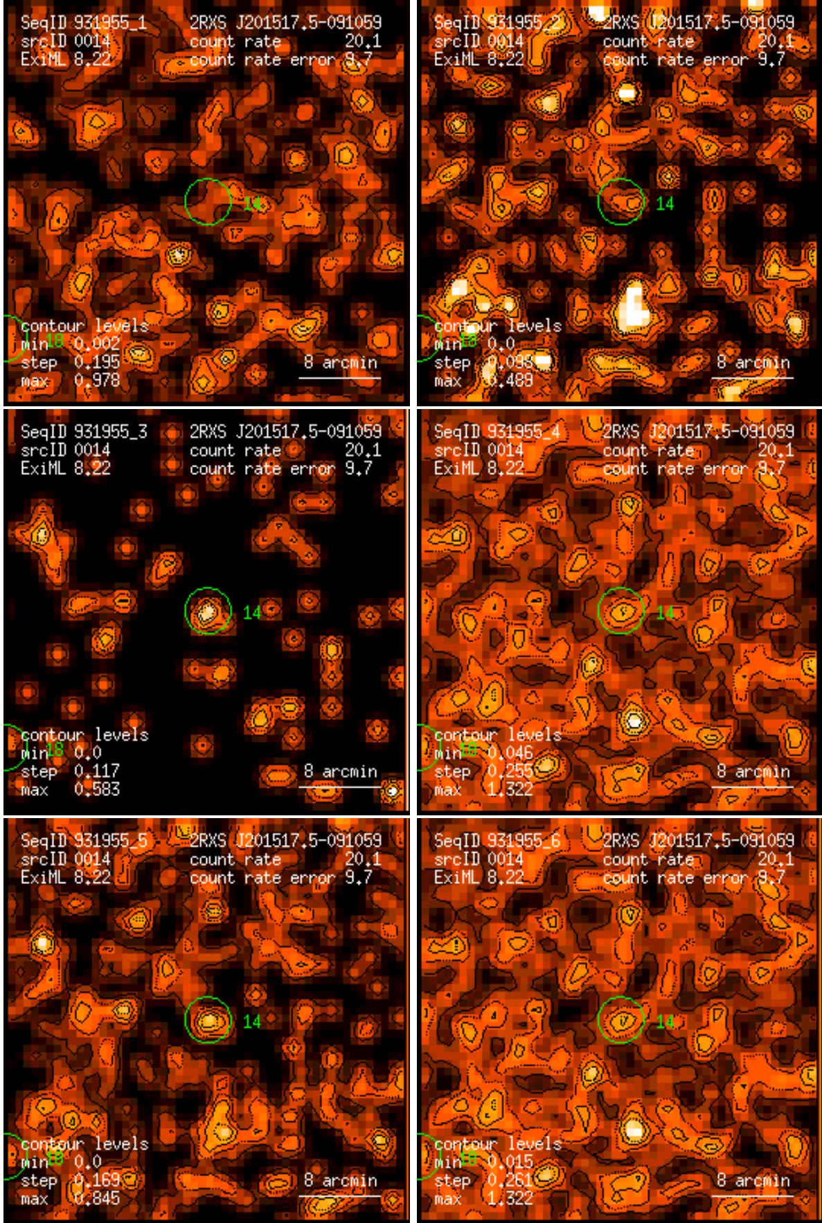
Figure 14: RASS 931955: detection 0014: band rate images, Gaussian filter: (1) PSPC channels 11 – 41, (2) 52 – 90, (3) 91 – 201, (4) 11 – 235, (5) 52 – 201, (6) 11 – 201. Broad band rates in counts/ks. Band rate contour levels in counts/ks/arcmin 2 .
