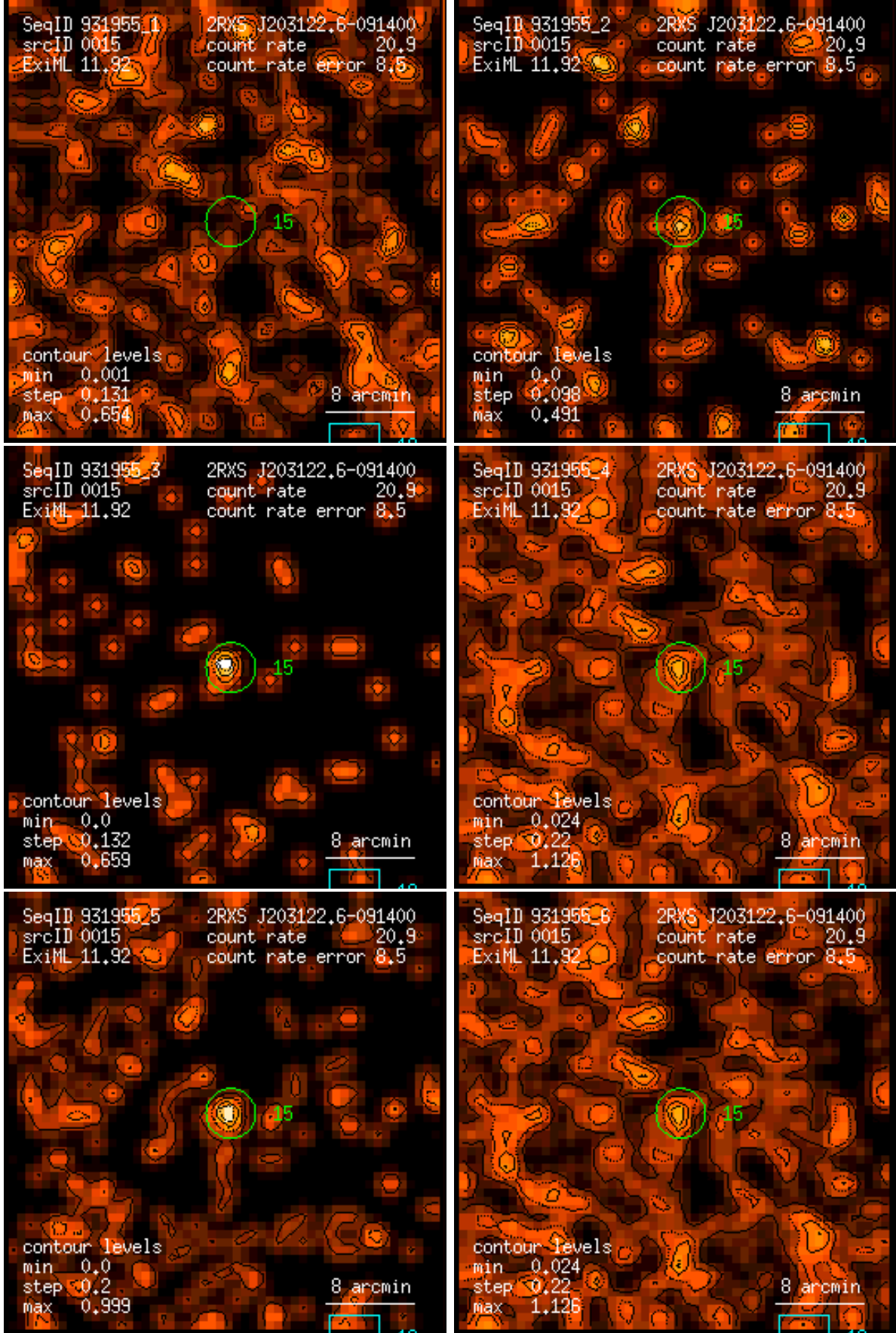
Figure 15: RASS 931955: detection 0015: band rate images, Gaussian filter: (1) PSPC channels 11 – 41, (2) 52 – 90, (3) 91 – 201, (4) 11 – 235, (5) 52 – 201, (6) 11 – 201. Broad band rates in counts/ks. Band rate contour levels in counts/ks/arcmin 2 .
