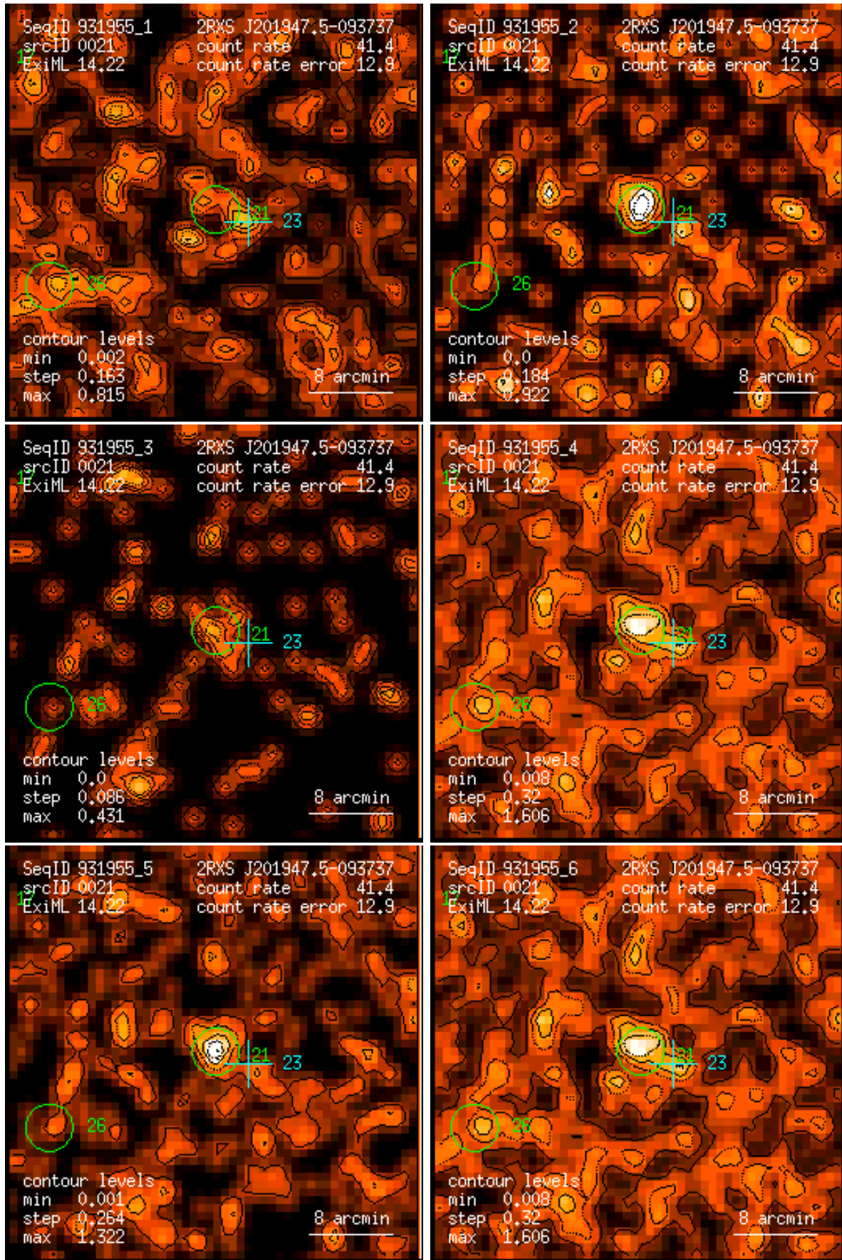
Figure 21: RASS 931955: detection 0021: band rate images, Gaussian filter: (1) PSPC channels 11 – 41, (2) 52 – 90, (3) 91 – 201, (4) 11 – 235, (5) 52 – 201, (6) 11 – 201. Broad band rates in counts/ks. Band rate contour levels in counts/ks/arcmin 2 .
