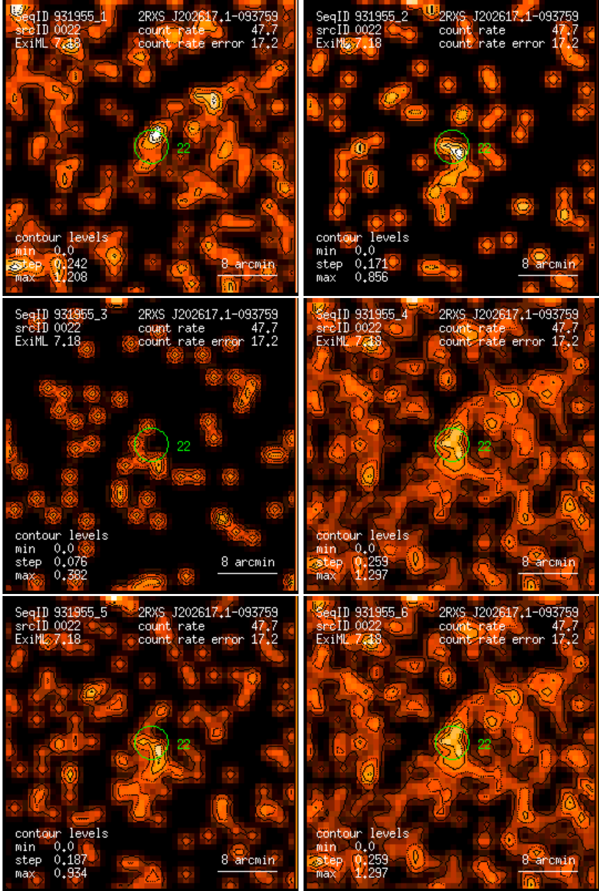
Figure 22: RASS 931955: detection 0022: band rate images, Gaussian filter: (1) PSPC channels 11 – 41, (2) 52 – 90, (3) 91 – 201, (4) 11 – 235, (5) 52 – 201, (6) 11 – 201. Broad band rates in counts/ks. Band rate contour levels in counts/ks/arcmin 2 .
