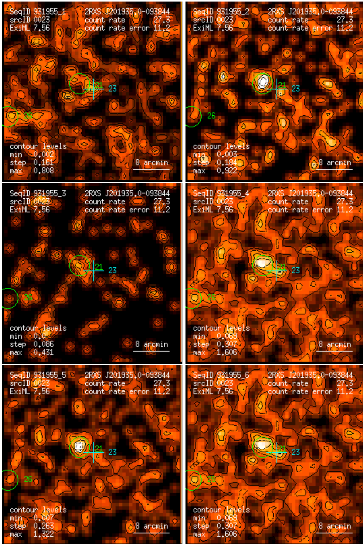
Figure 23: RASS 931955: detection 0023: band rate images, Gaussian filter: (1) PSPC channels 11 – 41, (2) 52 – 90, (3) 91 – 201, (4) 11 – 235, (5) 52 – 201, (6) 11 – 201. Broad band rates in counts/ks. Band rate contour levels in counts/ks/arcmin 2 .
