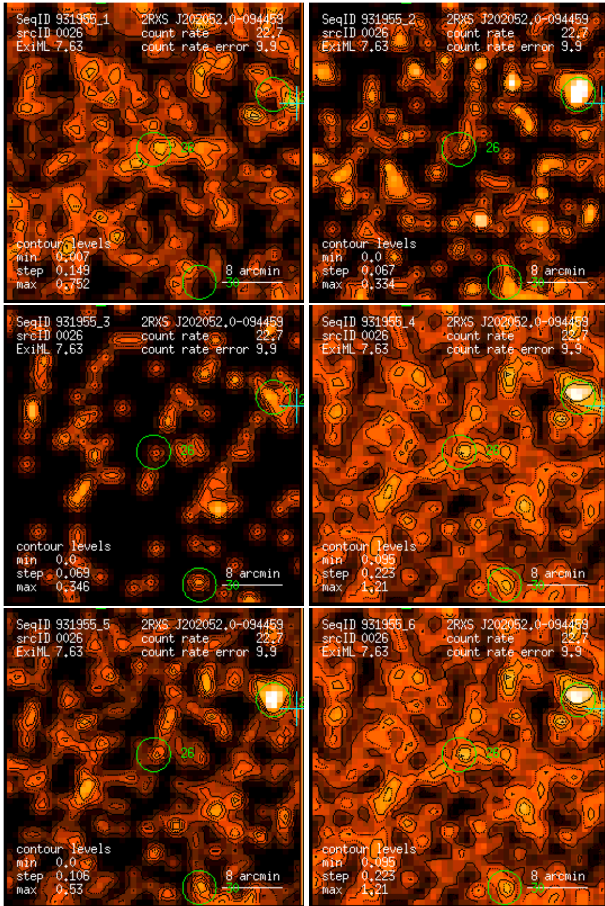
Figure 26: RASS 931955: detection 0026: band rate images, Gaussian filter: (1) PSPC channels 11 – 41, (2) 52 – 90, (3) 91 – 201, (4) 11 – 235, (5) 52 – 201, (6) 11 – 201. Broad band rates in counts/ks. Band rate contour levels in counts/ks/arcmin 2 .
