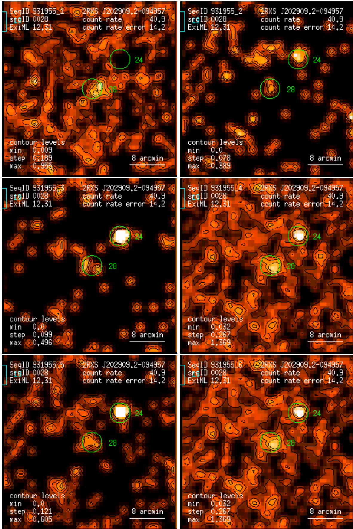
Figure 28: RASS 931955: detection 0028: band rate images, Gaussian filter: (1) PSPC channels 11 – 41, (2) 52 – 90, (3) 91 – 201, (4) 11 – 235, (5) 52 – 201, (6) 11 – 201. Broad band rates in counts/ks. Band rate contour levels in counts/ks/arcmin 2 .
