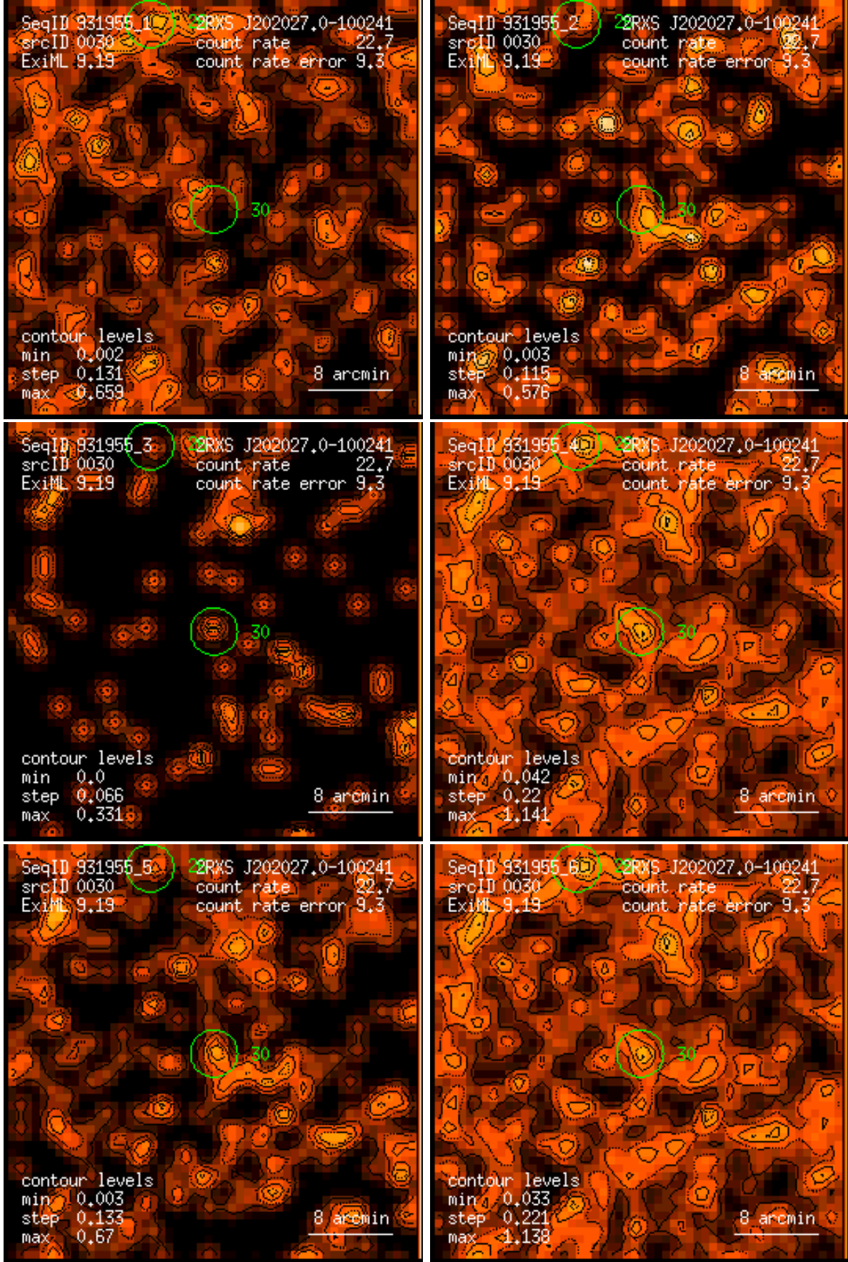
Figure 30: RASS 931955: detection 0030: band rate images, Gaussian filter: (1) PSPC channels 11 – 41, (2) 52 – 90, (3) 91 – 201, (4) 11 – 235, (5) 52 – 201, (6) 11 – 201. Broad band rates in counts/ks. Band rate contour levels in counts/ks/arcmin 2 .
