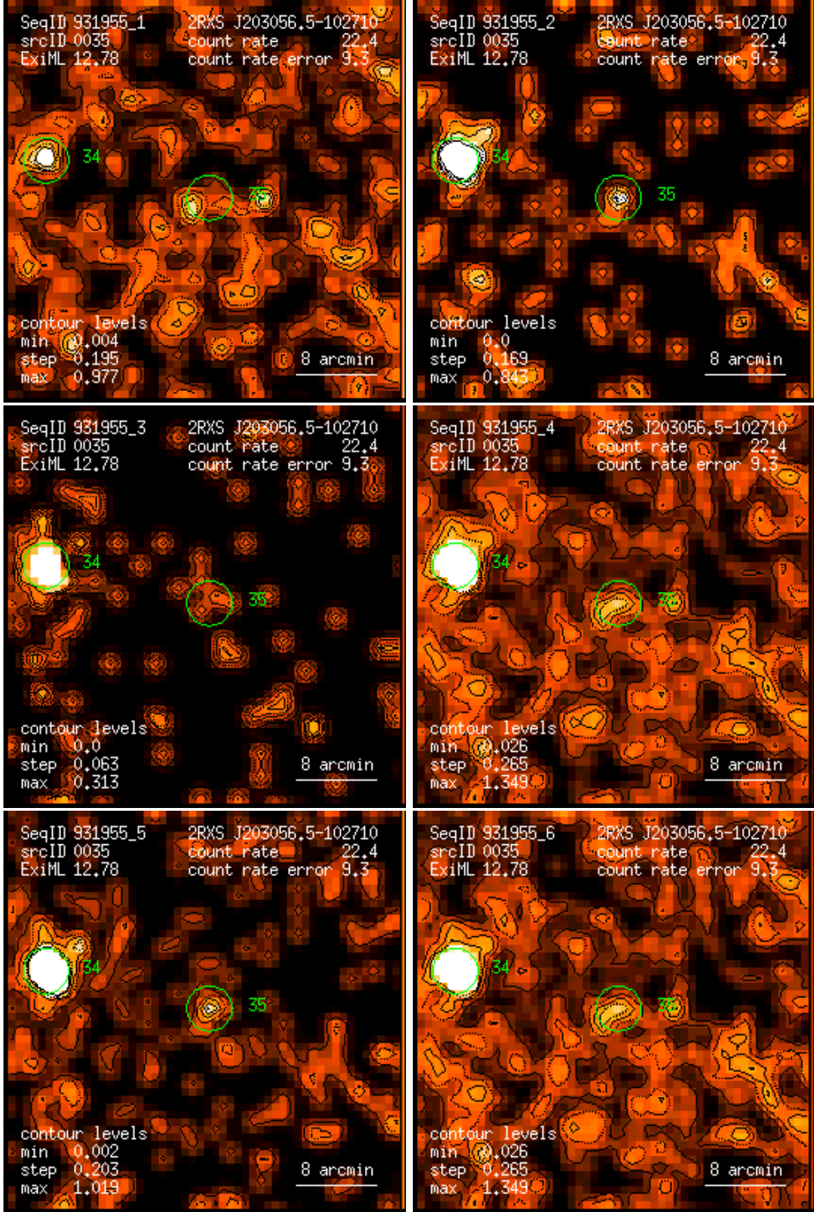
Figure 35: RASS 931955: detection 0035: band rate images, Gaussian filter: (1) PSPC channels 11 – 41, (2) 52 – 90, (3) 91 – 201, (4) 11 – 235, (5) 52 – 201, (6) 11 – 201. Broad band rates in counts/ks. Band rate contour levels in counts/ks/arcmin 2 .
