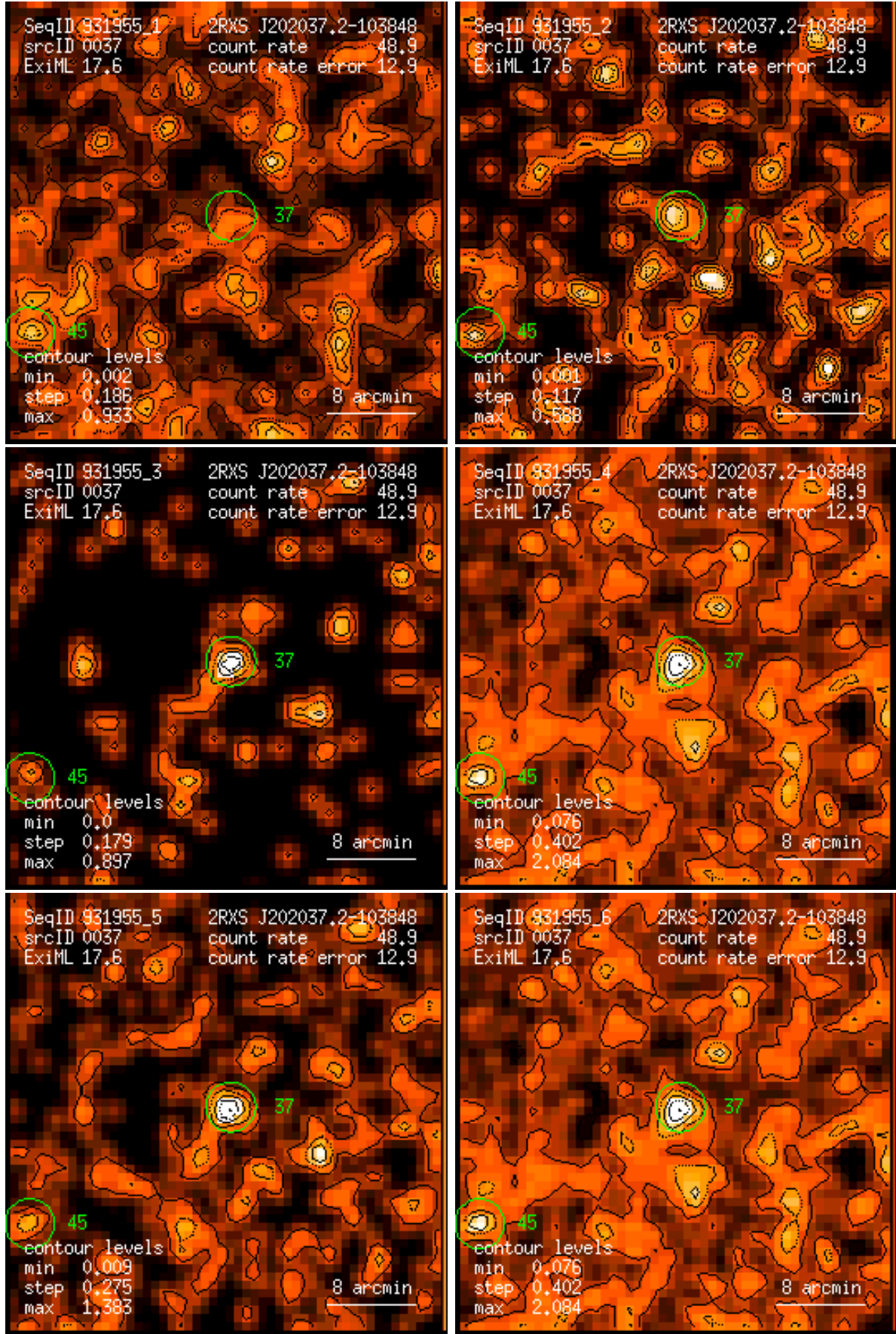
Figure 37: RASS 931955: detection 0037: band rate images, Gaussian filter: (1) PSPC channels 11 – 41, (2) 52 – 90, (3) 91 – 201, (4) 11 – 235, (5) 52 – 201, (6) 11 – 201. Broad band rates in counts/ks. Band rate contour levels in counts/ks/arcmin 2 .
