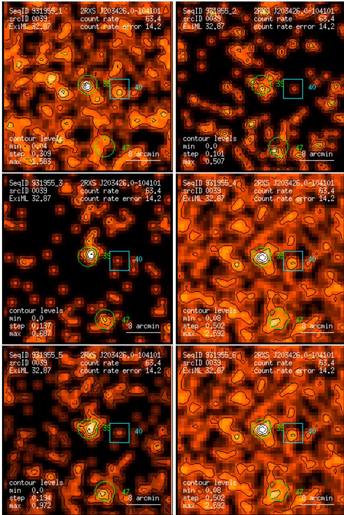
Figure 39: RASS 931955: detection 0039: band rate images, Gaussian filter: (1) PSPC channels 11 – 41, (2) 52 – 90, (3) 91 – 201, (4) 11 – 235, (5) 52 – 201, (6) 11 – 201. Broad band rates in counts/ks. Band rate contour levels in counts/ks/arcmin 2 .
