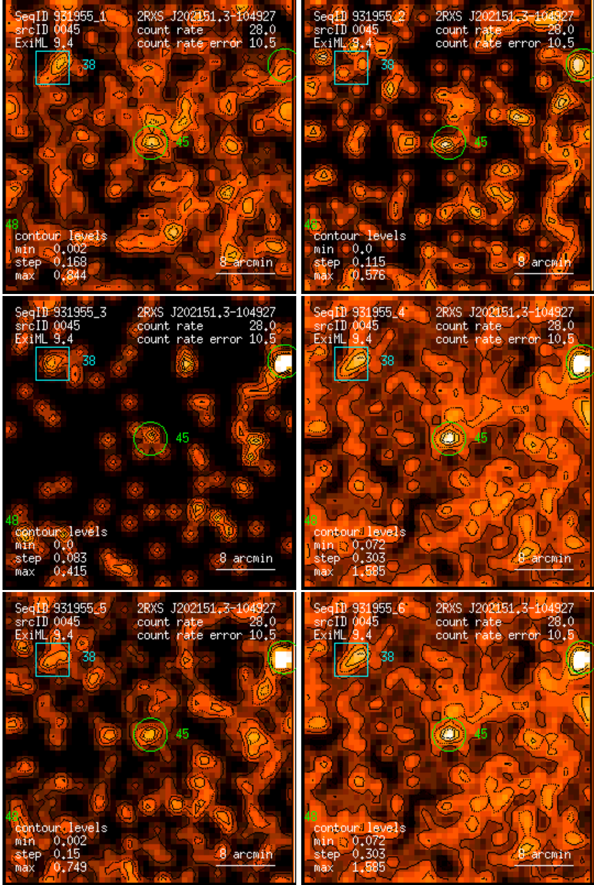
Figure 45: RASS 931955: detection 0045: band rate images, Gaussian filter: (1) PSPC channels 11 – 41, (2) 52 – 90, (3) 91 – 201, (4) 11 – 235, (5) 52 – 201, (6) 11 – 201. Broad band rates in counts/ks. Band rate contour levels in counts/ks/arcmin 2 .
