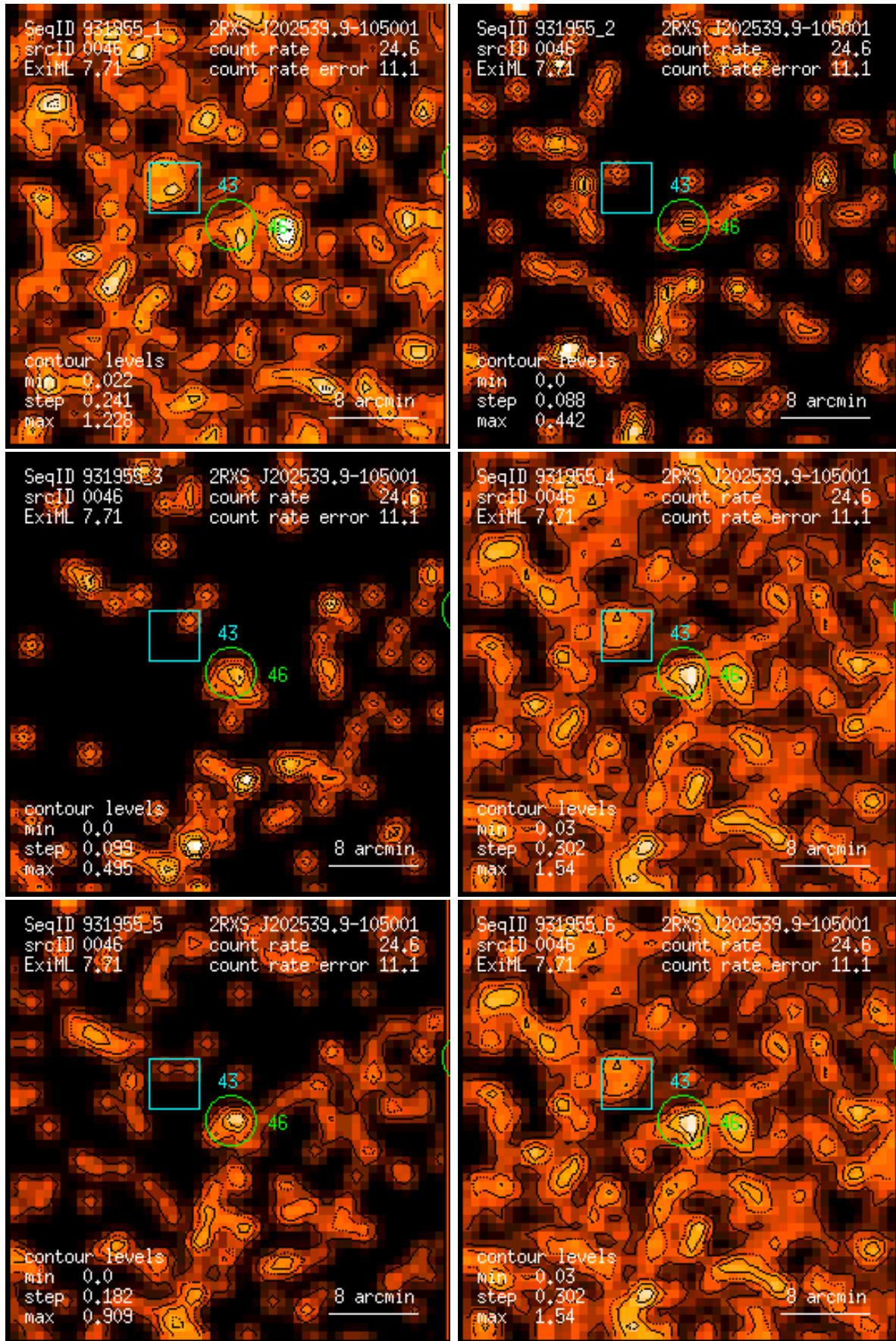
Figure 46: RASS 931955: detection 0046: band rate images, Gaussian filter: (1) PSPC channels 11 – 41, (2) 52 – 90, (3) 91 – 201, (4) 11 – 235, (5) 52 – 201, (6) 11 – 201. Broad band rates in counts/ks. Band rate contour levels in counts/ks/arcmin 2 .
