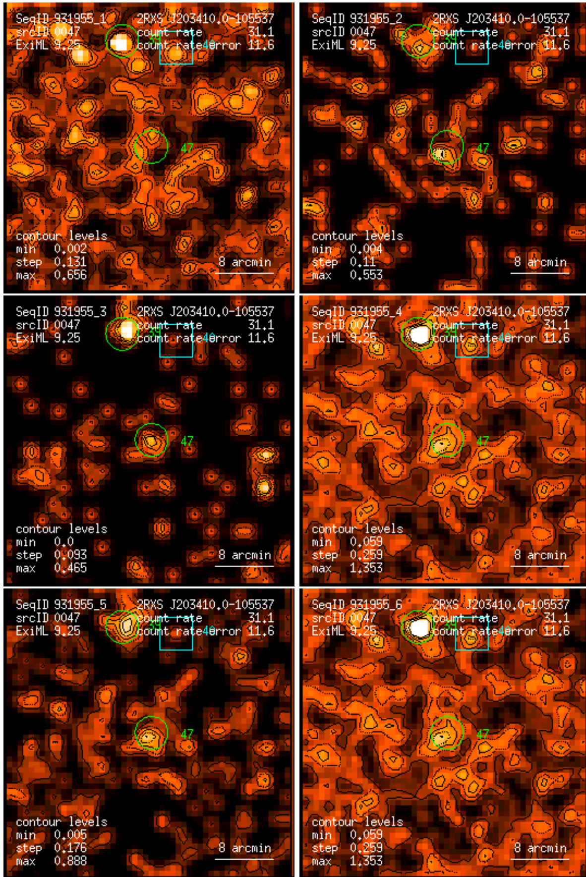
Figure 47: RASS 931955: detection 0047: band rate images, Gaussian filter: (1) PSPC channels 11 – 41, (2) 52 – 90, (3) 91 – 201, (4) 11 – 235, (5) 52 – 201, (6) 11 – 201. Broad band rates in counts/ks. Band rate contour levels in counts/ks/arcmin 2 .
