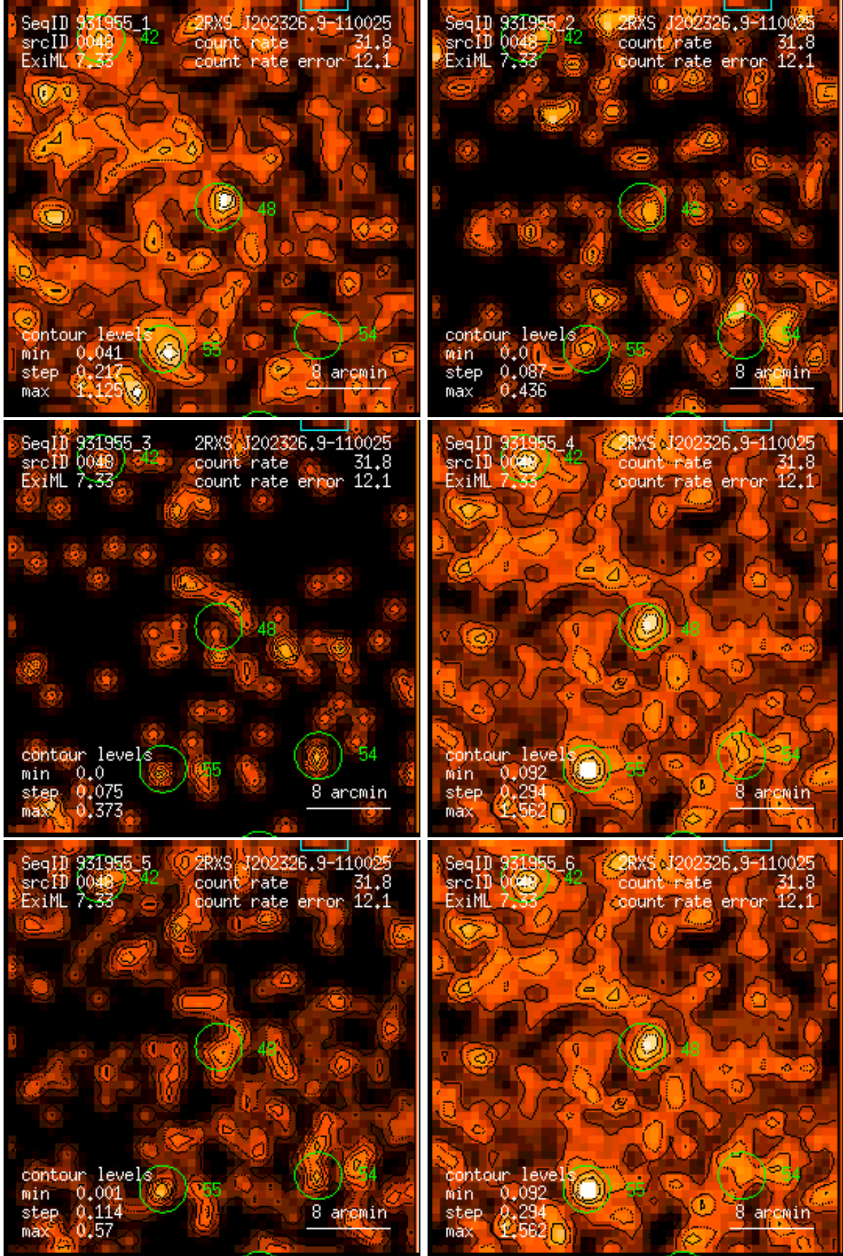
Figure 48: RASS 931955: detection 0048: band rate images, Gaussian filter: (1) PSPC channels 11 – 41, (2) 52 – 90, (3) 91 – 201, (4) 11 – 235, (5) 52 – 201, (6) 11 – 201. Broad band rates in counts/ks. Band rate contour levels in counts/ks/arcmin 2 .
