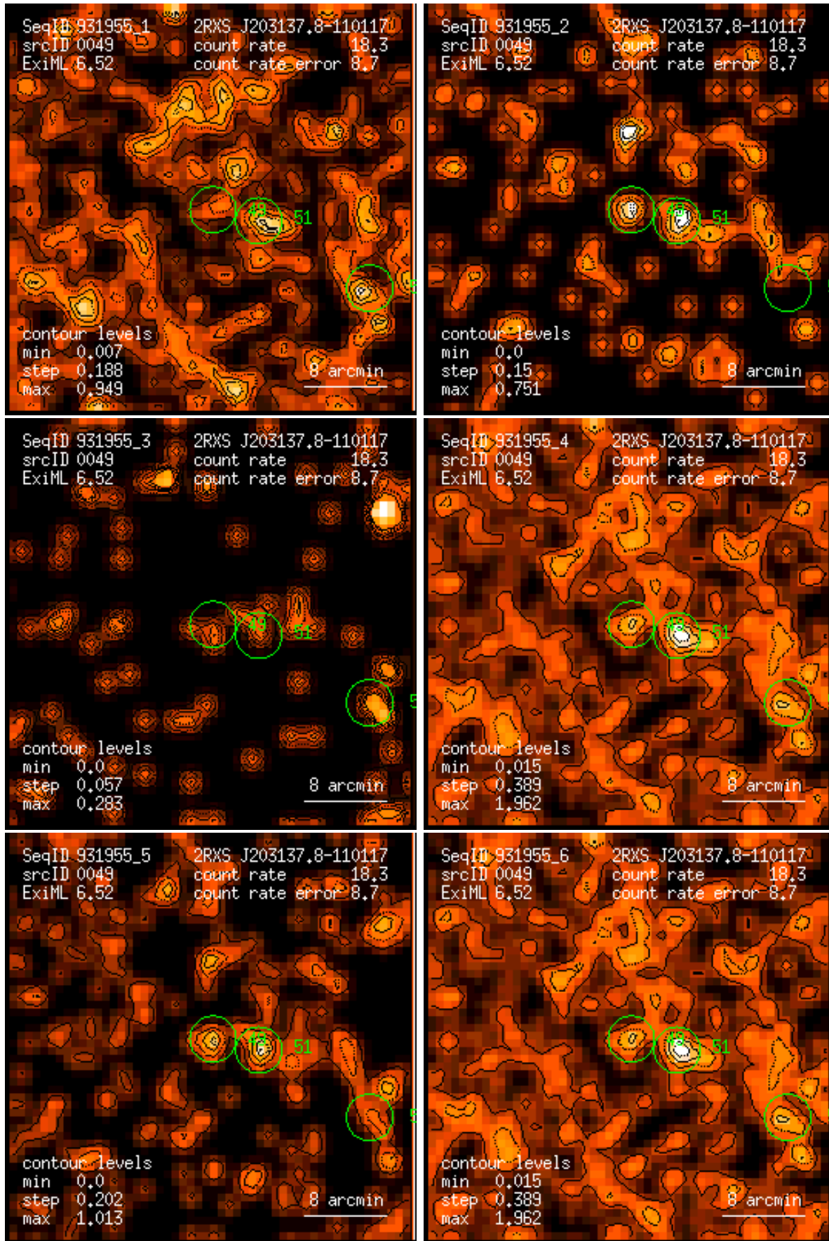
Figure 49: RASS 931955: detection 0049: band rate images, Gaussian filter: (1) PSPC channels 11 – 41, (2) 52 – 90, (3) 91 – 201, (4) 11 – 235, (5) 52 – 201, (6) 11 – 201. Broad band rates in counts/ks. Band rate contour levels in counts/ks/arcmin 2 .
