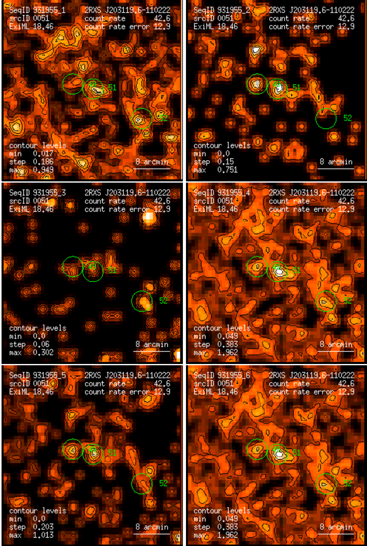
Figure 51: RASS 931955: detection 0051: band rate images, Gaussian filter: (1) PSPC channels 11 – 41, (2) 52 – 90, (3) 91 – 201, (4) 11 – 235, (5) 52 – 201, (6) 11 – 201. Broad band rates in counts/ks. Band rate contour levels in counts/ks/arcmin 2 .
