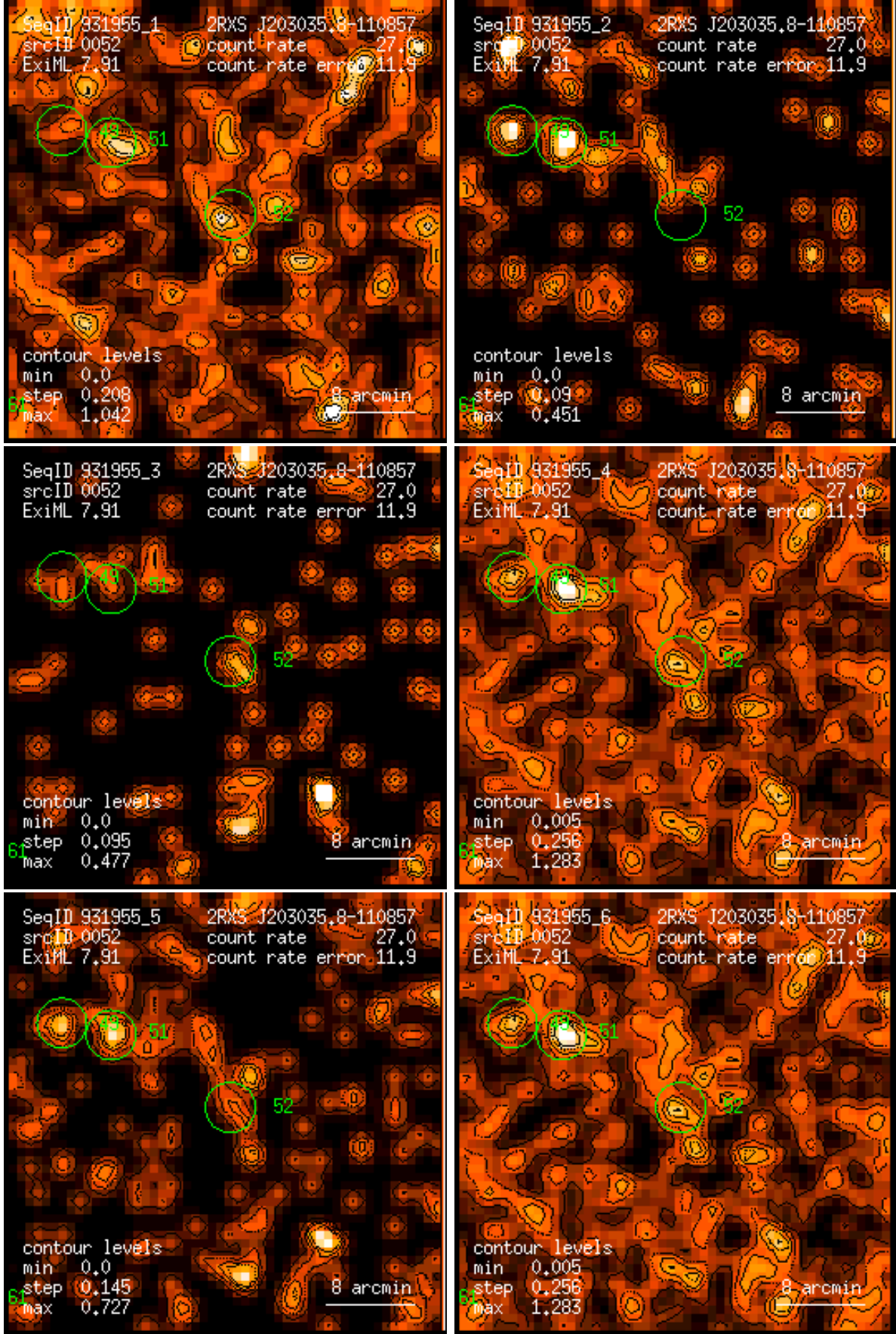
Figure 52: RASS 931955: detection 0052: band rate images, Gaussian filter: (1) PSPC channels 11 – 41, (2) 52 – 90, (3) 91 – 201, (4) 11 – 235, (5) 52 – 201, (6) 11 – 201. Broad band rates in counts/ks. Band rate contour levels in counts/ks/arcmin 2 .
