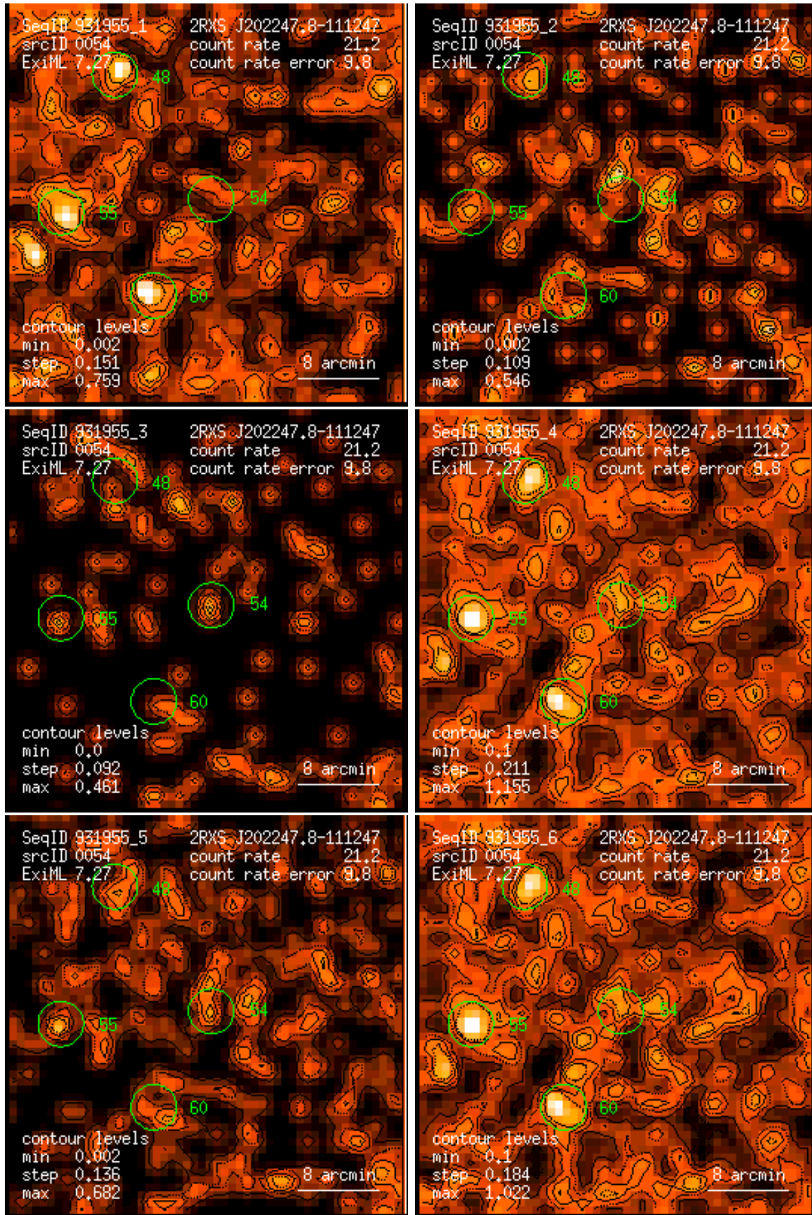
Figure 54: RASS 931955: detection 0054: band rate images, Gaussian filter: (1) PSPC channels 11 – 41, (2) 52 – 90, (3) 91 – 201, (4) 11 – 235, (5) 52 – 201, (6) 11 – 201. Broad band rates in counts/ks. Band rate contour levels in counts/ks/arcmin 2 .
