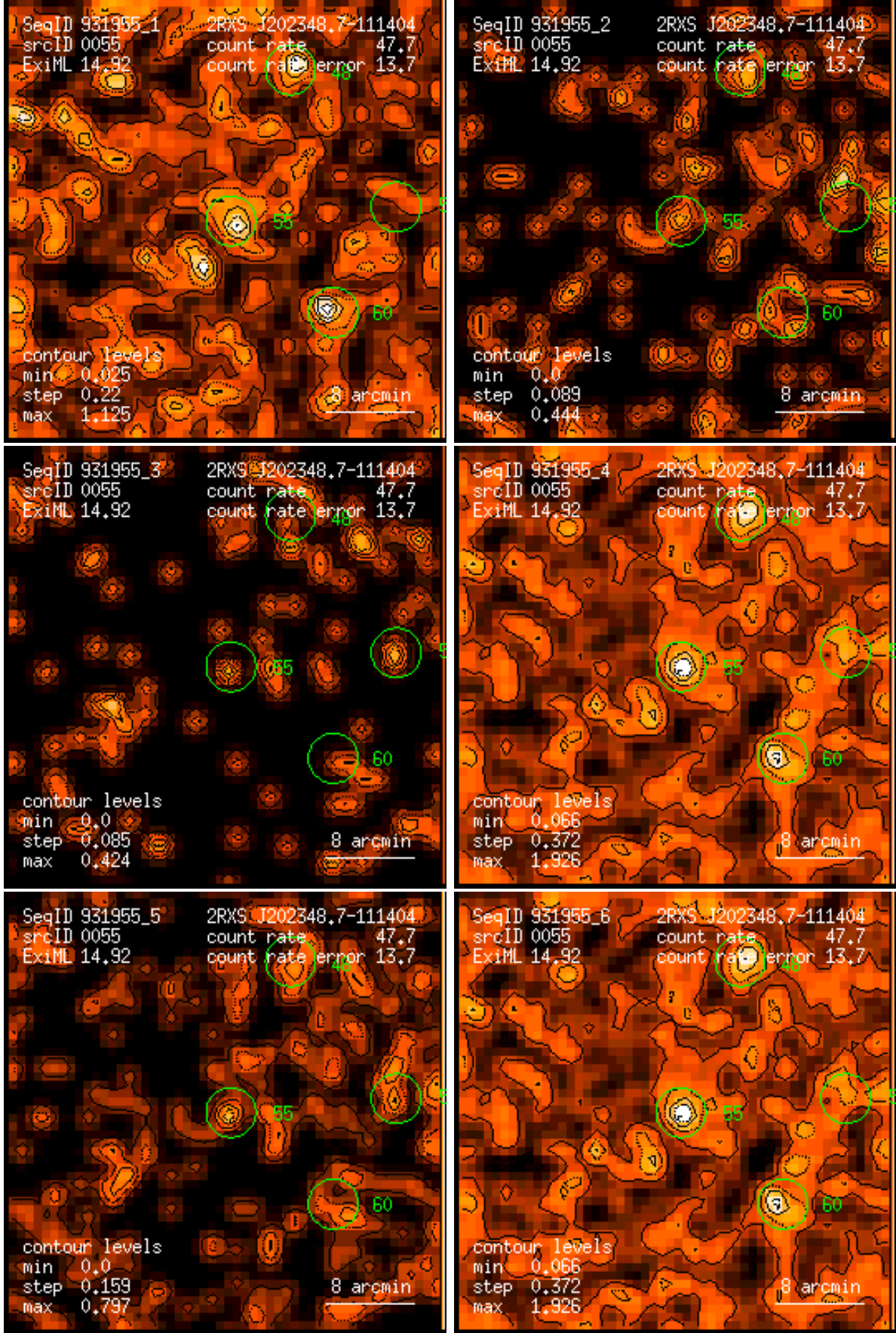
Figure 55: RASS 931955: detection 0055: band rate images, Gaussian filter: (1) PSPC channels 11 – 41, (2) 52 – 90, (3) 91 – 201, (4) 11 – 235, (5) 52 – 201, (6) 11 – 201. Broad band rates in counts/ks. Band rate contour levels in counts/ks/arcmin 2 .
