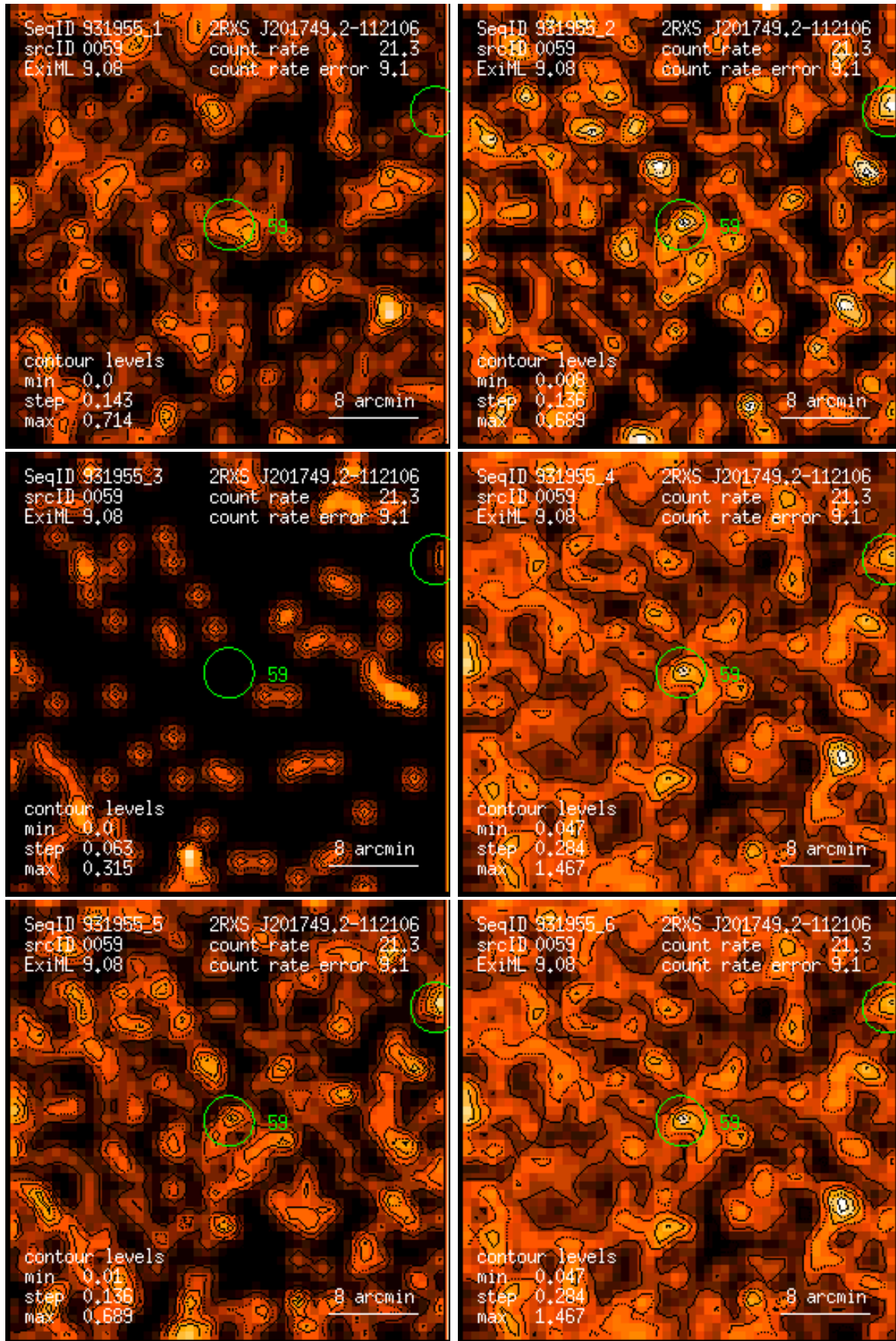
Figure 59: RASS 931955: detection 0059: band rate images, Gaussian filter: (1) PSPC channels 11 – 41, (2) 52 – 90, (3) 91 – 201, (4) 11 – 235, (5) 52 – 201, (6) 11 – 201. Broad band rates in counts/ks. Band rate contour levels in counts/ks/arcmin 2 .
