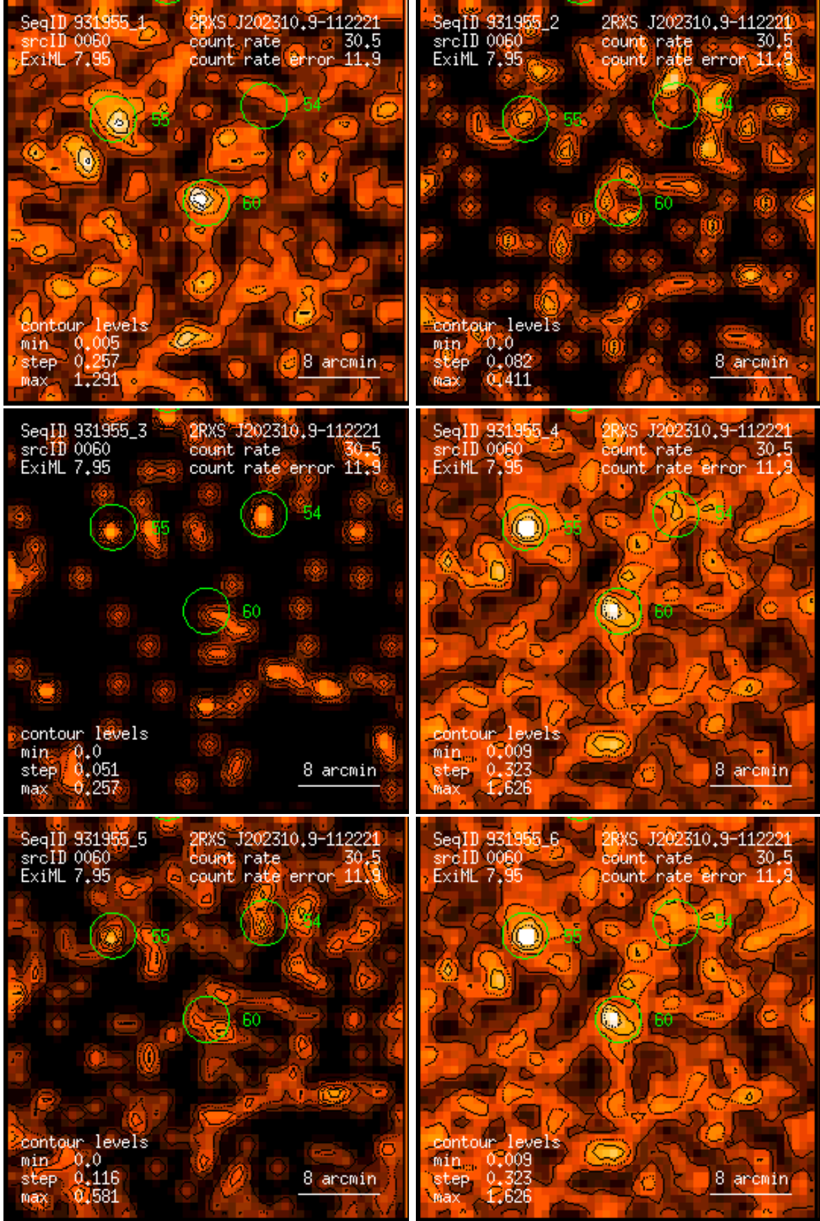
Figure 60: RASS 931955: detection 0060: band rate images, Gaussian filter: (1) PSPC channels 11 – 41, (2) 52 – 90, (3) 91 – 201, (4) 11 – 235, (5) 52 – 201, (6) 11 – 201. Broad band rates in counts/ks. Band rate contour levels in counts/ks/arcmin 2 .
