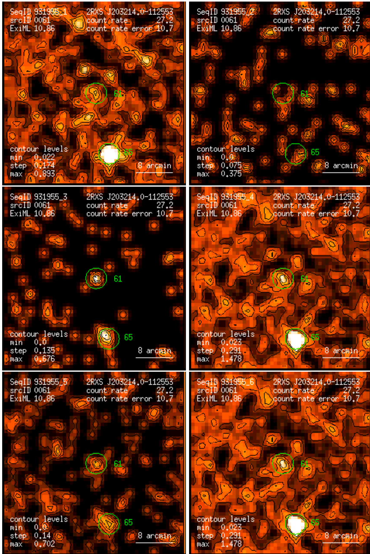
Figure 61: RASS 931955: detection 0061: band rate images, Gaussian filter: (1) PSPC channels 11 – 41, (2) 52 – 90, (3) 91 – 201, (4) 11 – 235, (5) 52 – 201, (6) 11 – 201. Broad band rates in counts/ks. Band rate contour levels in counts/ks/arcmin 2 .
