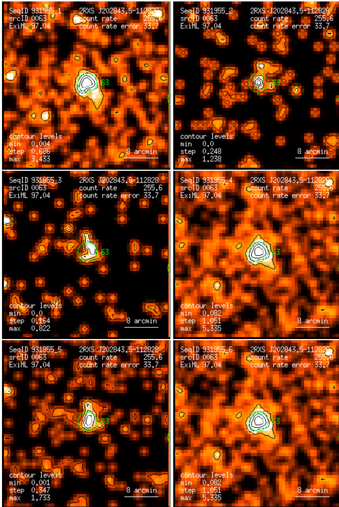
Figure 63: RASS 931955: detection 0063: band rate images, Gaussian filter: (1) PSPC channels 11 – 41, (2) 52 – 90, (3) 91 – 201, (4) 11 – 235, (5) 52 – 201, (6) 11 – 201. Broad band rates in counts/ks. Band rate contour levels in counts/ks/arcmin 2 .
