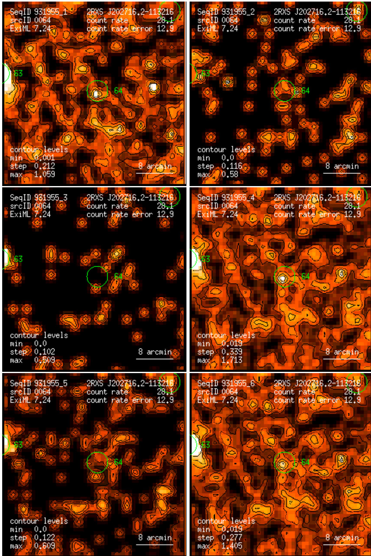
Figure 64: RASS 931955: detection 0064: band rate images, Gaussian filter: (1) PSPC channels 11 – 41, (2) 52 – 90, (3) 91 – 201, (4) 11 – 235, (5) 52 – 201, (6) 11 – 201. Broad band rates in counts/ks. Band rate contour levels in counts/ks/arcmin 2 .
